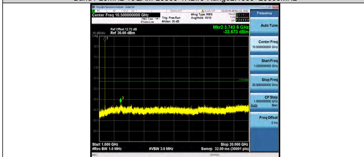
Band4-20MHz-16QAM-20300-1RB#0-Range2:1000~20000MHz
