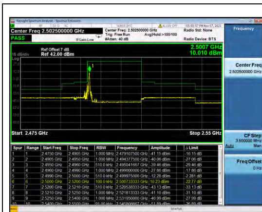
1-DC_5A_N7A-15KHZ-10MHZ+20MHZ-N/A+DFT-PI2BPSK-MID+LOW-N/A-EDGE_1 RB_RIGHT-PASS
