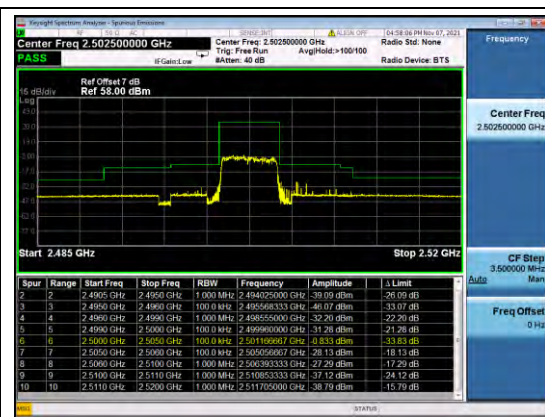
1-DC_5A_N7A-15KHZ-10MHZ+5MHZ-N/A+ DFT-PI2BPSK-MID+LOW-N/A-OUTER_FUL L--PASS
