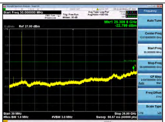
1-DC_5A_N7A-15KHZ-10MHZ+15MHZ-N/A+ DFT-PI2BPSK-MID+MID-N/A-EDGE_1RB_LE FT-30-9000--PASS
