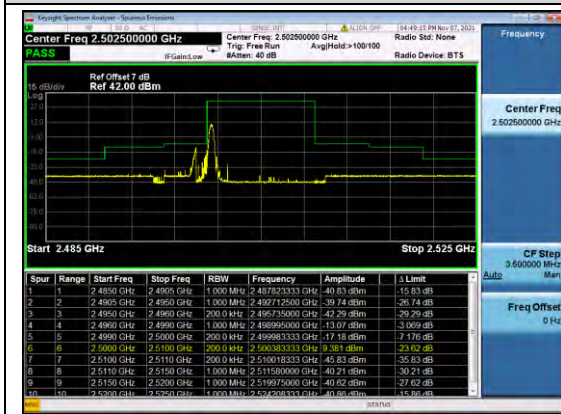
1-DC_5A_N7A-15KHZ-10MHZ+10MHZ-N/A+ DFT-PI2BPSK -MID+LOW-N/A-EDGE_1RB_LEFT--PASS
