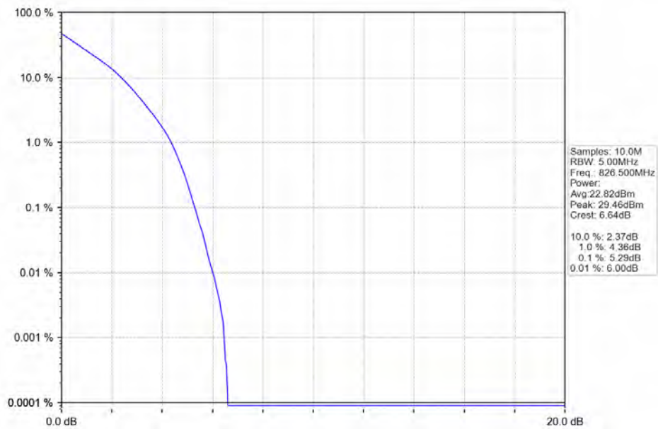
Band 5 5MHz QPSK LCH 826.5MHz RB 25_0 NTV
