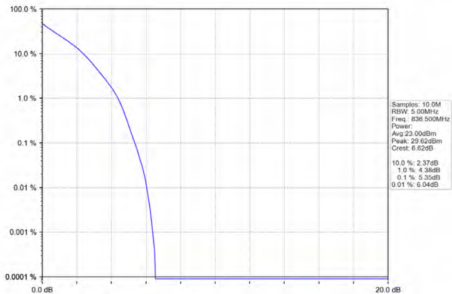
Band 5 5MHz QPSK MCH 836.5MHz RB 25_0 NTV
