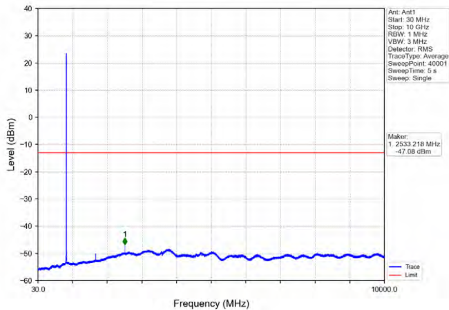
Band 5 5MHz 64QAM HCH 846.5MHz RB 1 24 NTV
