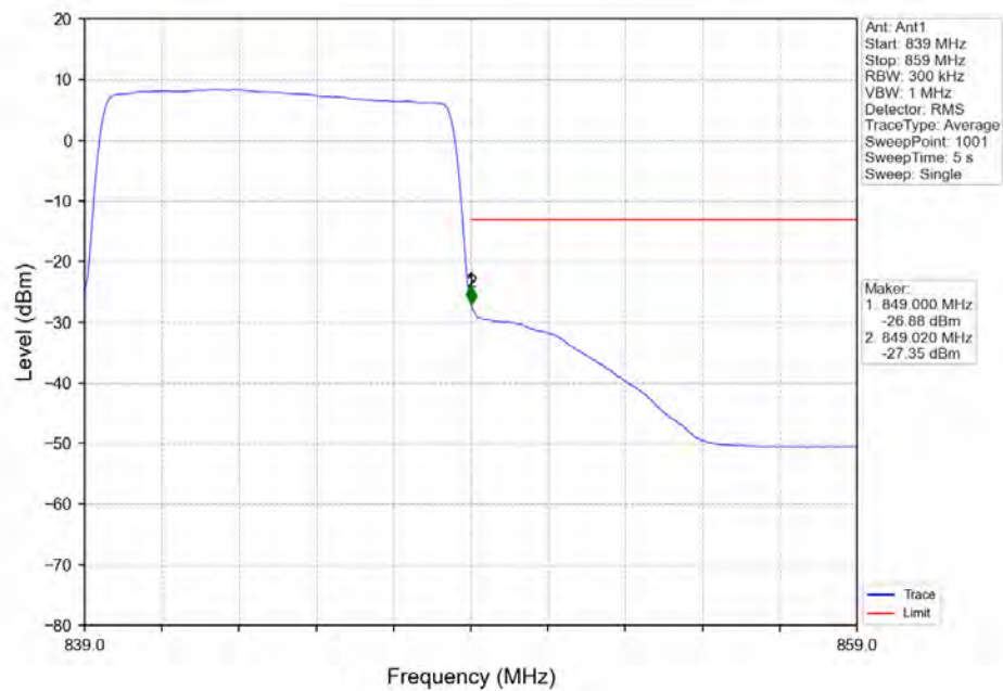
Band26_10MHz_16QAM_HCH_844MHz_RB_50_0_NTNV
