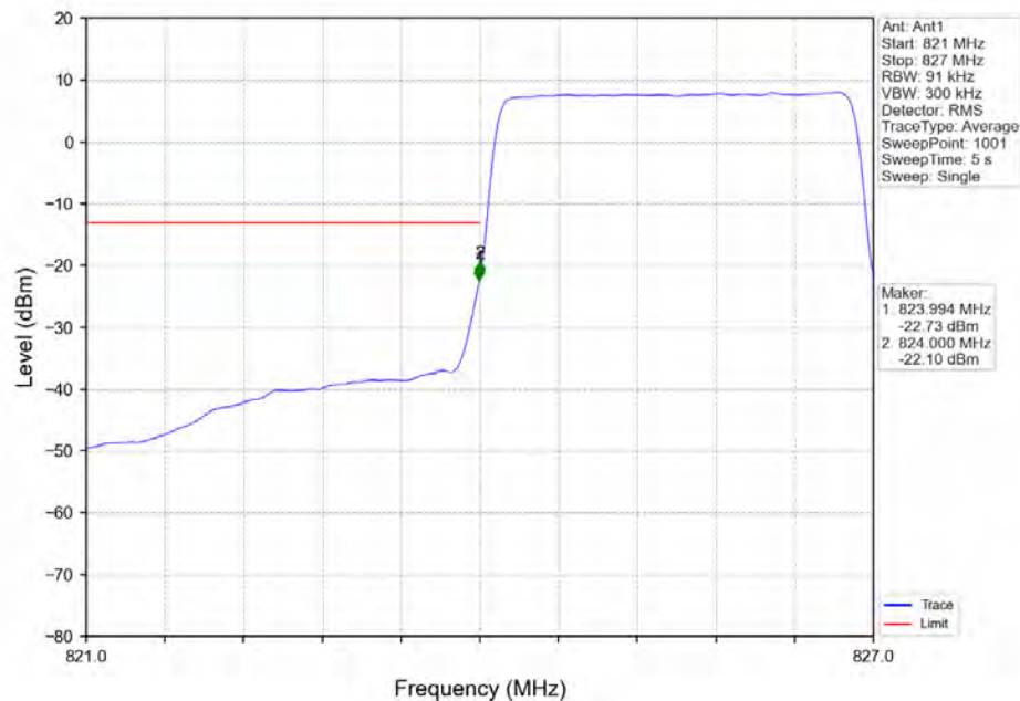
Band26_3MHz_64QAM_LCH_825.5MHz_RB_15_0_NTNV
