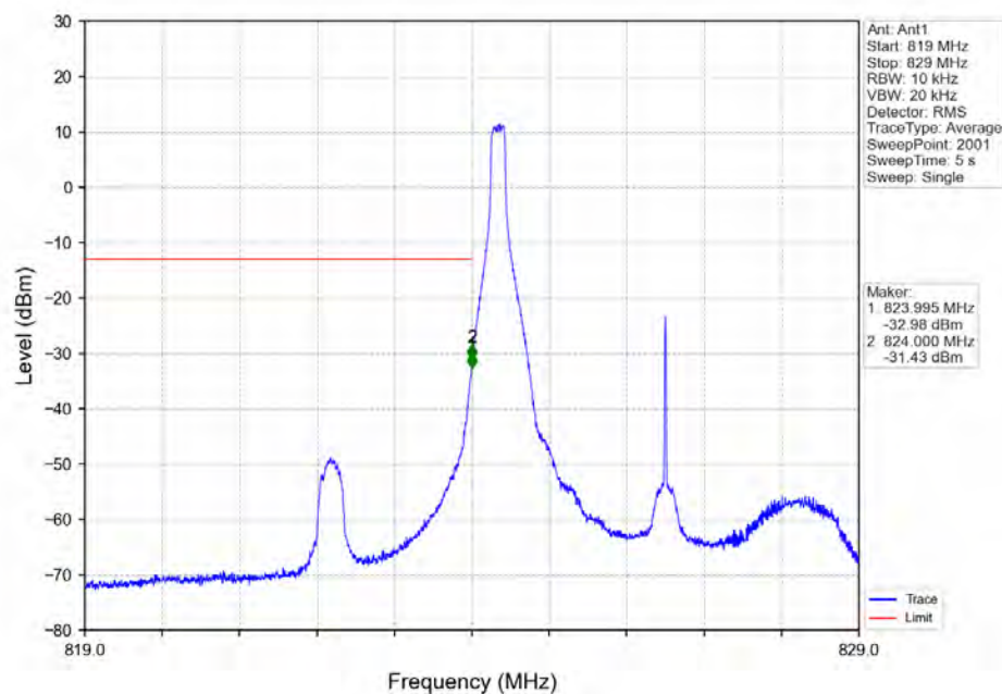
Band_5_5MHz_16QAM_LCH_826.5MHz_RB_1_0_NTNV
