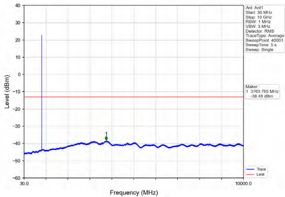
Band26_5MHz_16QAM_HCH_846.5MHz_RB_1_0_NTNV
