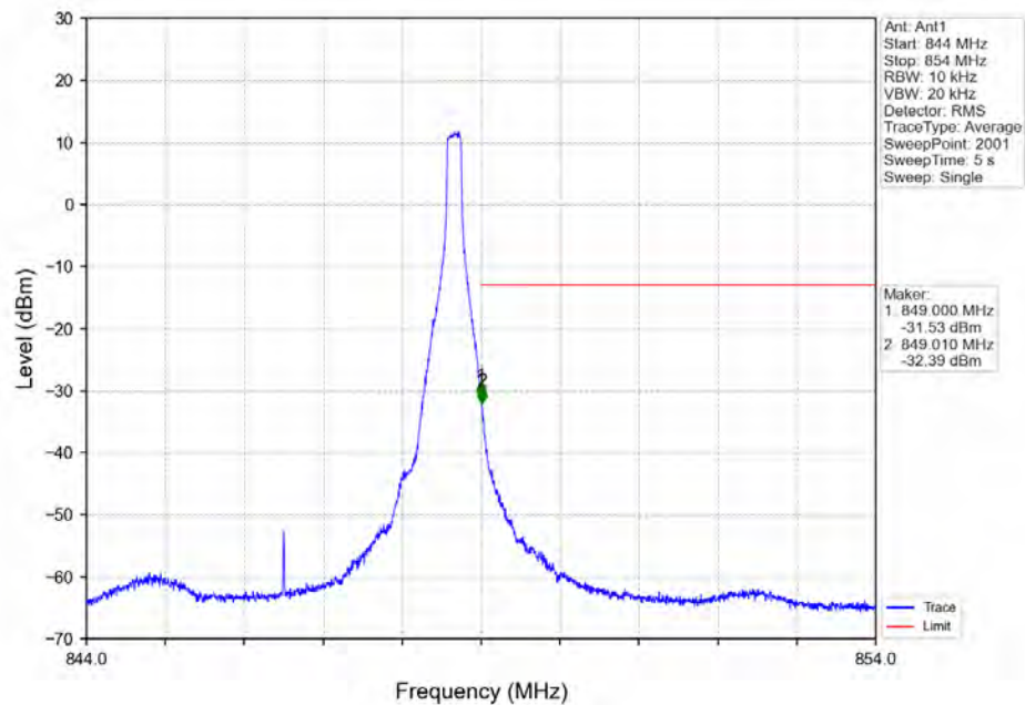
Band26_5MHz_64QAM_HCH_846.5MHz_RB_1_24_NTNV
