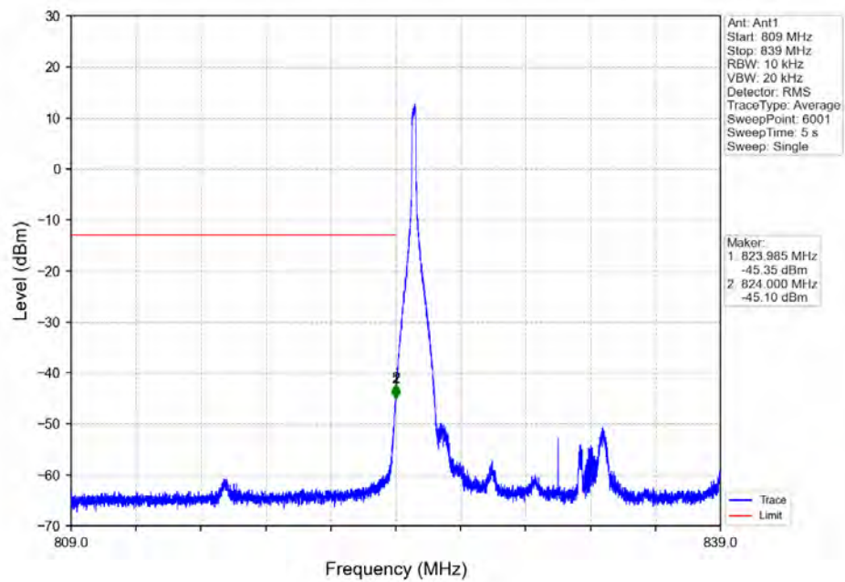
Band26_15MHz_QPSK_LCH_831.5MHz_RB_1_0_NTNV
