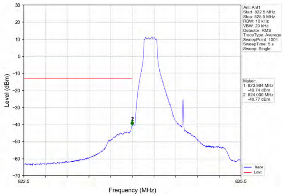
Band26_1.4MHz_16QAM_LCH_824.7MHz_RB_1_0_NTNV
