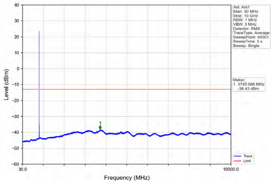
Band26_15MHz_QPSK_LCH_831.5MHz_RB_1_0_NTNV
