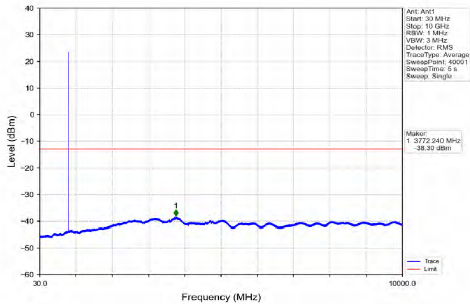
Band26_3MHz_QPSK_LCH_825.5MHz_RB_15_0_NTNV
