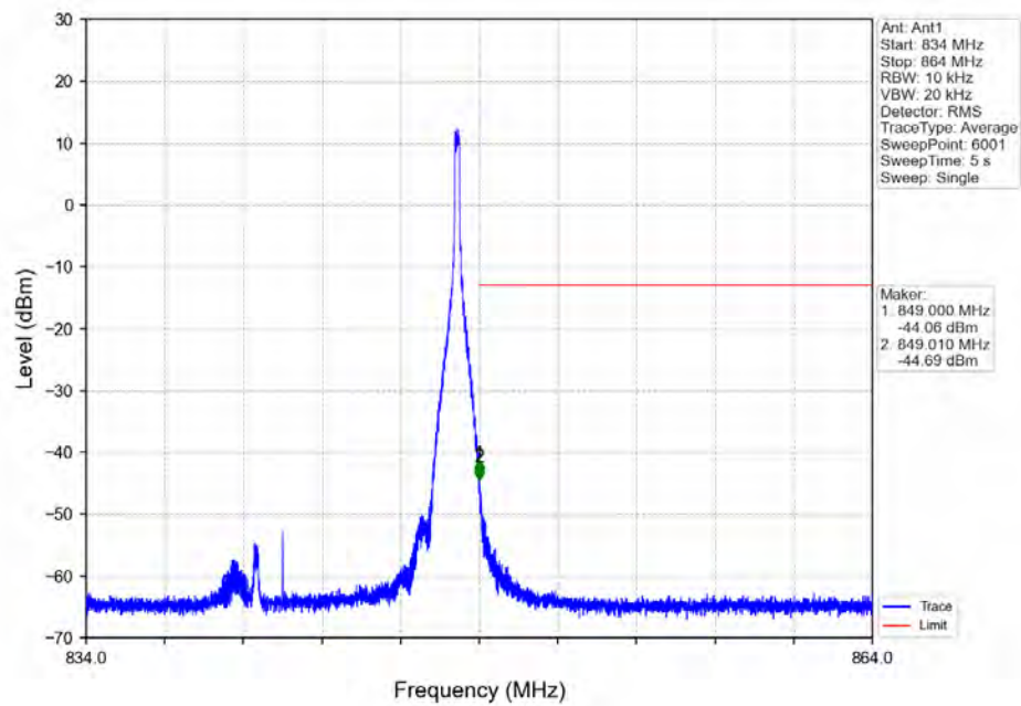
Band26_15MHz_16QAM_HCH_841.5MHz_RB_75_0_NTNV
