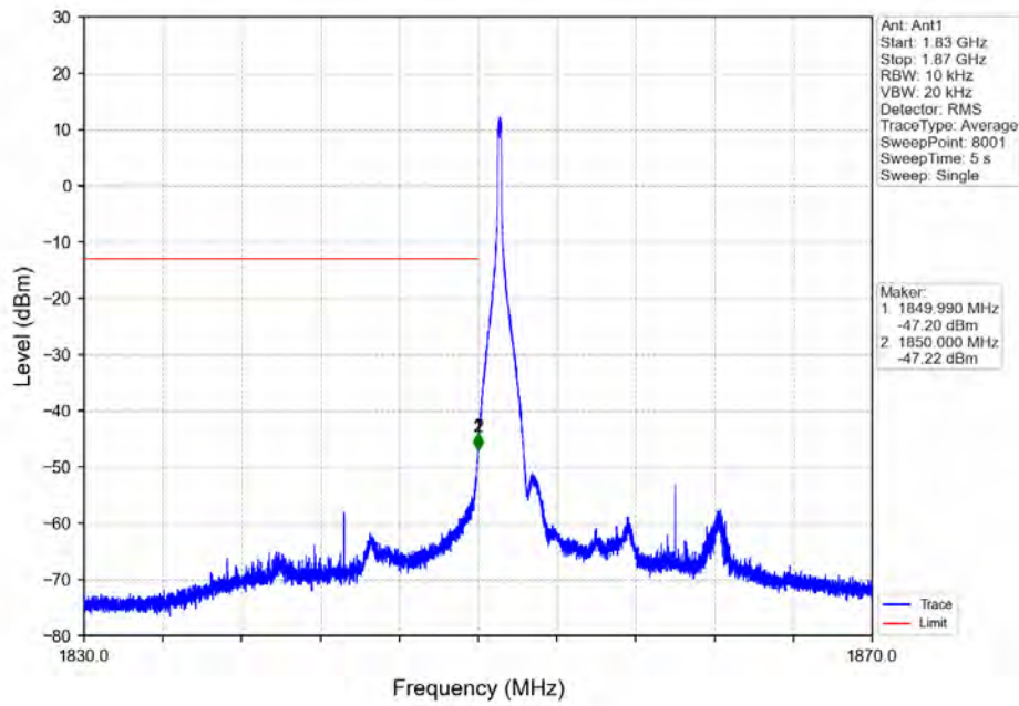
Band_25_20MHz_64QAM_LCH_1860MHz_RB_1_0_NTNV
