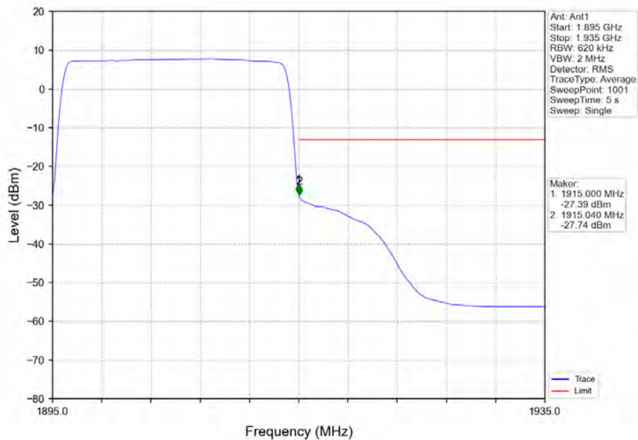
Band_25_20MHz_16QAM_HCH_1905MHz_RB_100_0_NTNV
