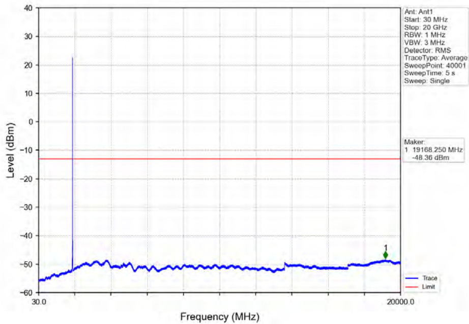
Band_25_15MHz_64QAM_HCH_1907.5MHz_RB_1_74_NTNV
