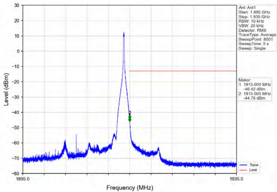
Band_25_20MHz_16QAM_HCH_1905MHz_RB_100_0_NTNV
