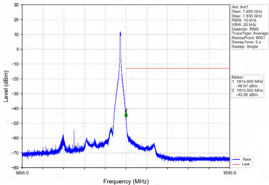
Band_25_20MHz_64QAM_HCH_1905MHz_RB_1_99_NTNV
