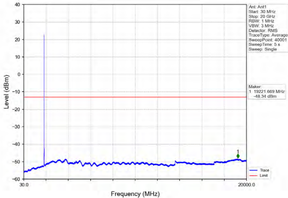
Band_25_20MHz_64QAM_LCH_1860MHz_RB_1_0_NTNV
