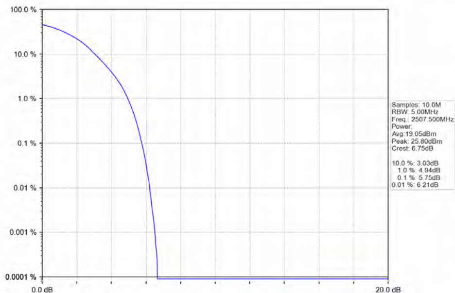
Band7_15MHz_QPSK_LCH_2507.5MHz_RB_75_0_NTNV
