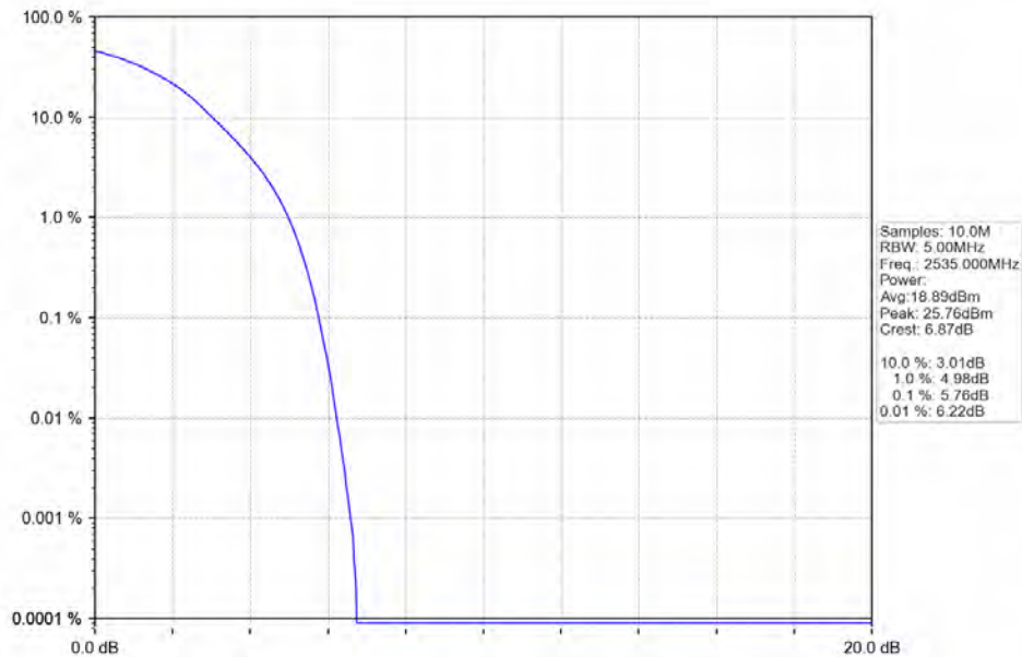
Band7_15MHz_QPSK_MCH_2535MHz_RB_75_0_NTNV
