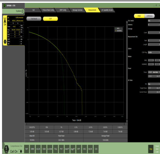
1-N25-PC3-15-40-L-15-NS_01-DFT-256QAM-Outer_ Full-216@0-6.99
