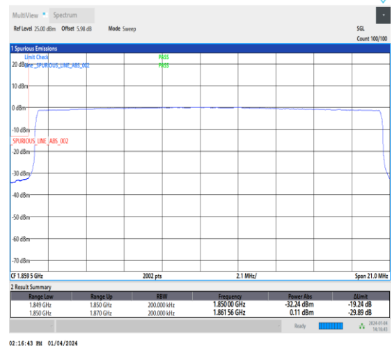
1-N25-15-20-L-6-CP-QPSK-Outer_Full-106@0-Ant1-1-seegraph-PASS-see graph
