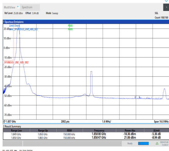
1-N25-15-15-L-1-DFT-PI2BPSK-Edge_1RB_Left-1@0-Ant1-1-seegraph-PASS-see graph
