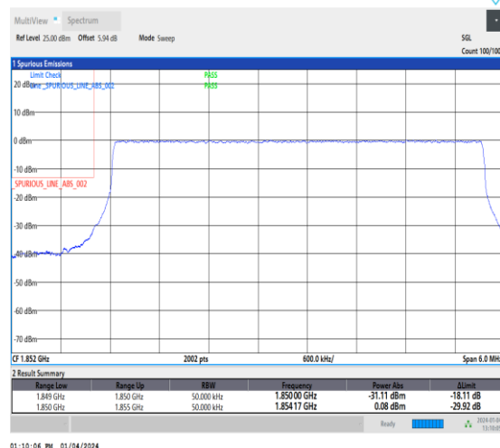
1-N25-15-5-L-6-CP-QPSK-Outer_Full-25@0-Ant1-1 1-seegraph-PASS-see graph
