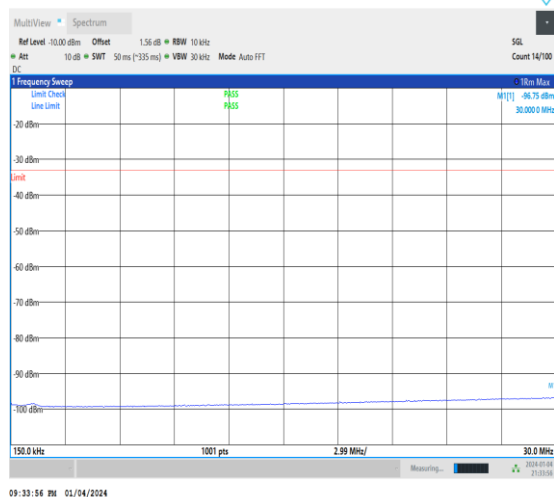
1-N25-15-40-L-1-DFT-PI2BPSK-Inner_1RB_Left-1@ 1-0.15-30-Ant1-30.00--96.75--33-PASS
