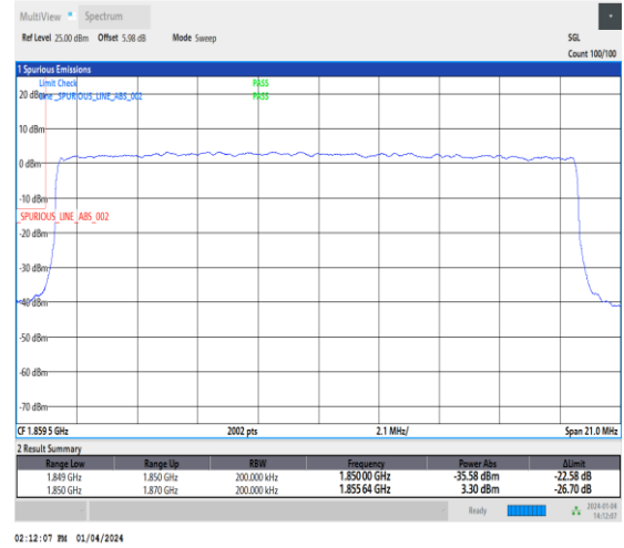
1-N25-15-20-L-3-DFT-PI2BPSK-Outer_Full-100@0-Ant1-1-seegraph-PASS-see graph
