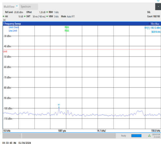
1-N25-15-40-L-1-DFT-PI2BPSK-Inner_1RB_Left-1 @1-0.009-0.15-Ant1-0.06--100.12--43-PASS
