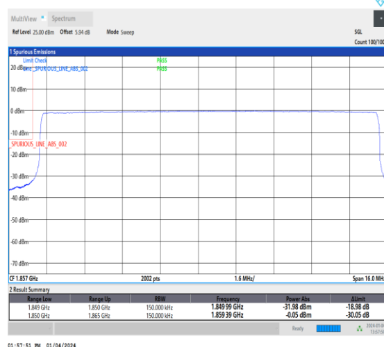
1-N25-15-15-L-6-CP-QPSK-Outer_Full-79@0-Ant1-1-seegraph-PASS-see graph
