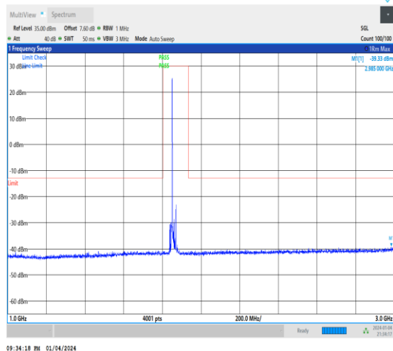
1-N25-15-40-L-1-DFT-PI2BPSK-Inner_1RB_Left-1@ 1-1000-3000-Ant1-2985.00--39.33--13-PASS
