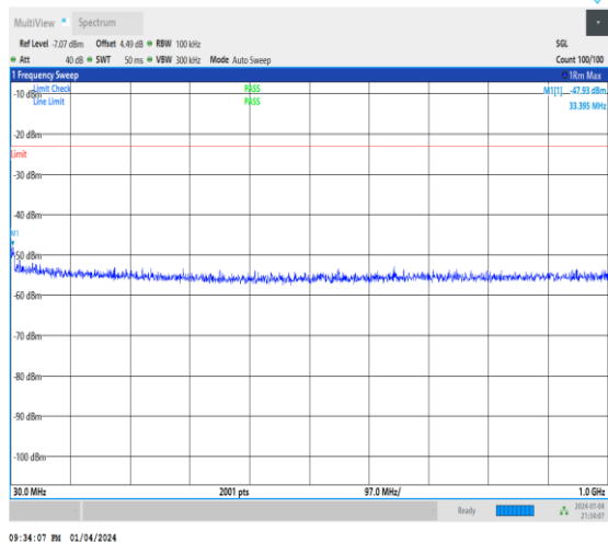
1-N25-15-40-L-1-DFT-PI2BPSK-Inner_1RB_Left-1 @1-30-1000-Ant1-33.40--47.93--23-PASS
