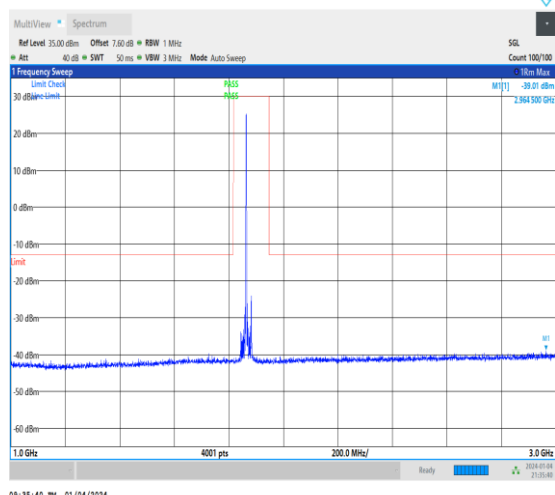
1-N25-15-40-M-1-DFT-PI2BPSK-Inner_1RB_Left-1@ 1-1000-3000-Ant1-2964.50--39.01--13-PASS
