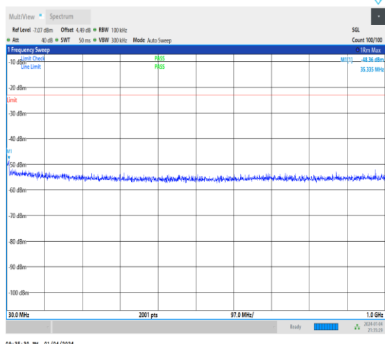
1-N25-15-40-M-1-DFT-PI2BPSK-Inner_1RB_Left-1 @ 1-30-1000-Ant1-35.34--48.36--23-PASS
