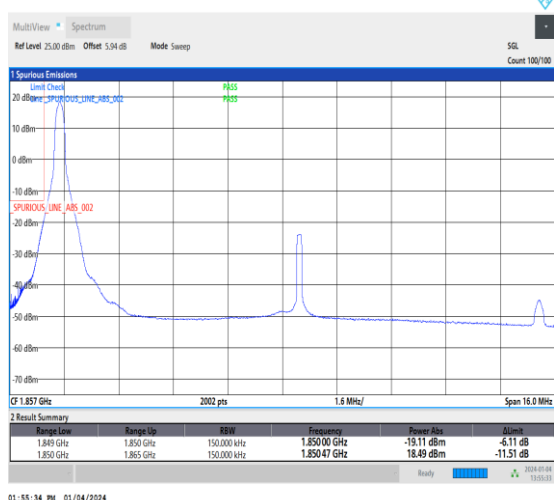
1-N25-15-15-L-4-CP-QPSK-Edge_1RB_Left-1@0-Ant1-1-seegraph-PASS-see graph
