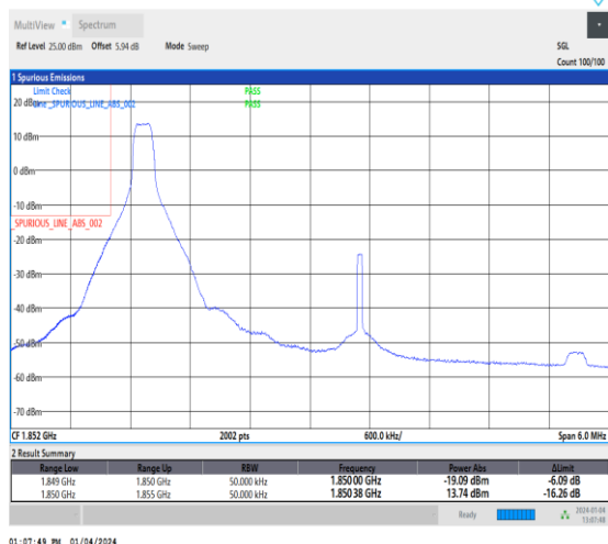
1-N25-15-5-L-4-CP-QPSK-Edge_1RB_Left-1@0-Ant1-1 1-seegraph-PASS-see graph
