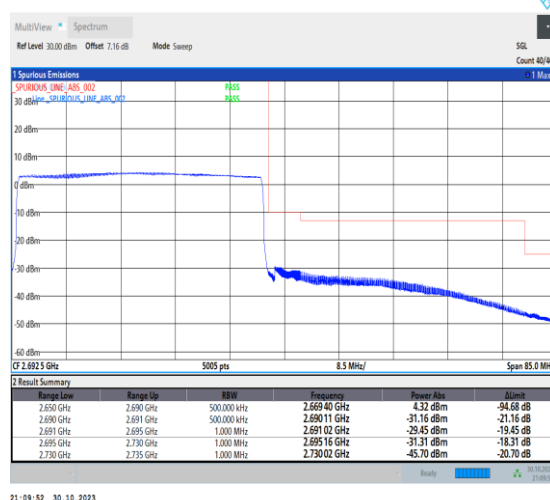
1-N41-30-40-H-6-CP-QPSK-Outer_Full-106@0-Ant1-1--PASS-see graph
