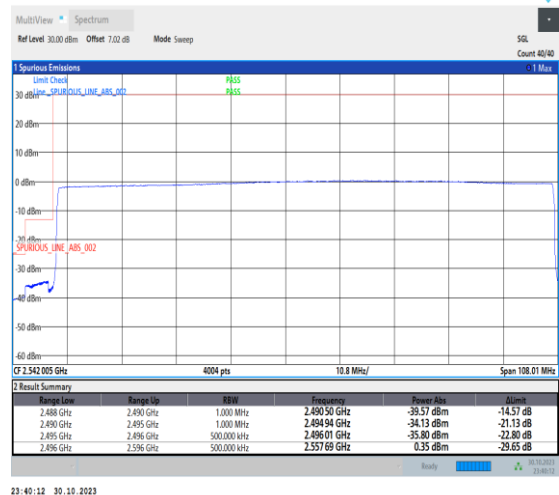
1-N41-30-100-L-6-CP-QPSK-Outer_Full-273@0-Ant1-1--PASS-see graph
