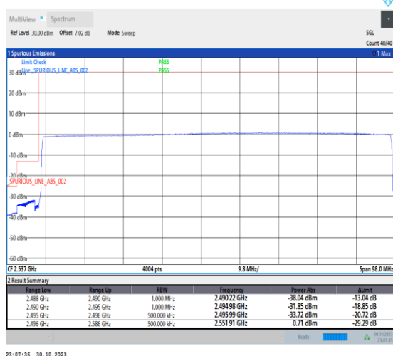
1-N41-30-90-L-6-CP-QPSK-Outer_Full-245@0-Ant1-1--PASS-see graph
