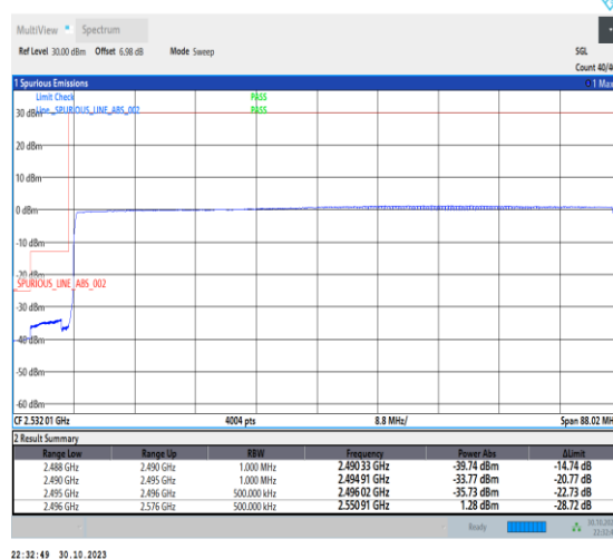
1-N41-30-80-L-6-CP-QPSK-Outer_Full-217@0-Ant1-1--PASS-see graph
