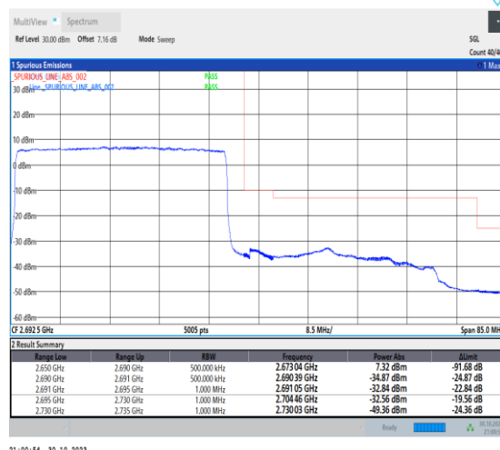
1-N41-30-40-H-3-DFT-PI2BPSK-Outer_Full-100@0-Ant1-1--PASS-see graph
