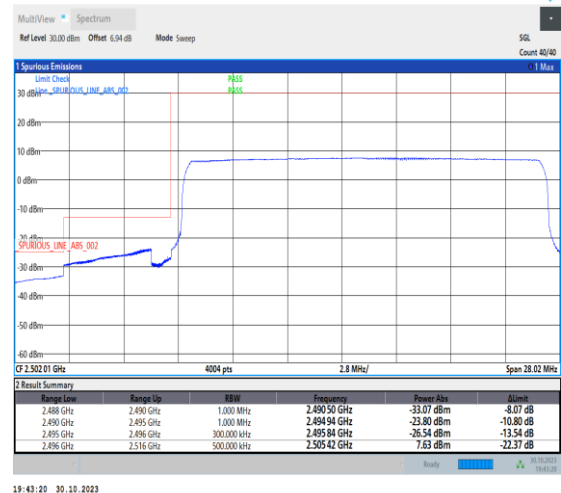
1-N41-30-20-L-6-CP-QPSK-Outer_Full-51@0-Ant1-1--PASS-see graph
