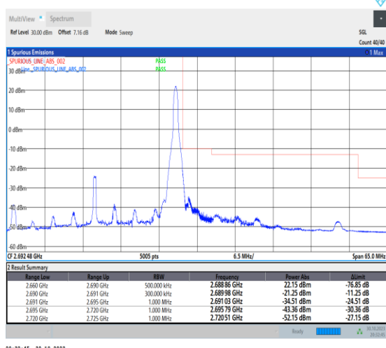
1-N41-30-30-H-5-CP-QPSK-Edge_1RB_Right-1@77-Ant1-1--PASS-see graph
