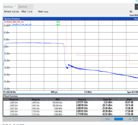
1-N41-30-30-H-6-CP-QPSK-Outer_Full-78@0-Ant1-1--PASS-see graph
