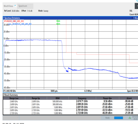
1-N41-30-30-H-3-DFT-PI2BPSK-Outer_Full-75@0-Ant1-1--PASS-see graph
