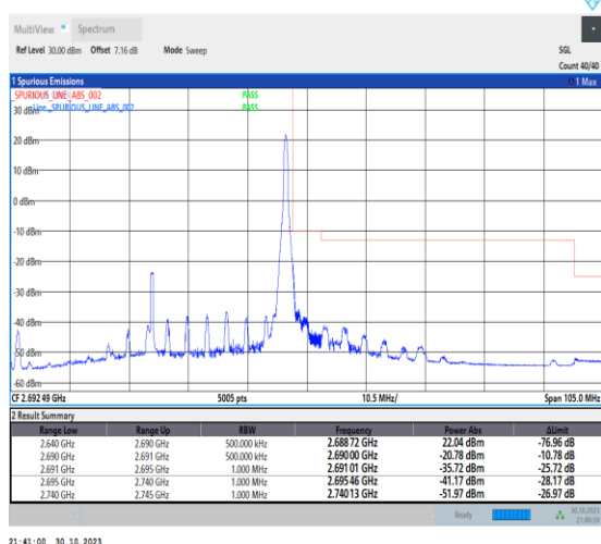
1-N41-30-50-H-5-CP-QPSK-Edge_1RB_Right-1@132-Ant1-1--PASS-see graph
