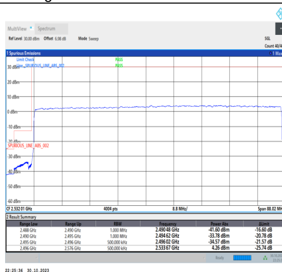
1-N41-30-80-L-3-DFT-PI2BPSK-Outer_Full-216@0-Ant1-1--PASS-see graph
