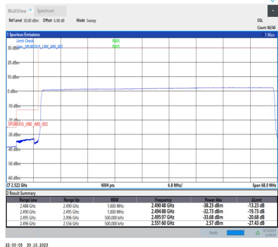
1-N41-30-60-L-6-CP-QPSK-Outer_Full-162@0-Ant1-1--PASS-see graph
