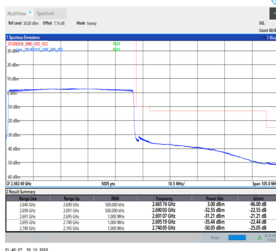
1-N41-30-50-H-6-CP-QPSK-Outer_Full-133@0-Ant1-1--PASS-see graph
