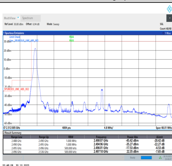
1-N41-30-40-L-4-CP-QPSK-Edge_1RB_Left-1@0-Ant1-1--PASS-see graph
