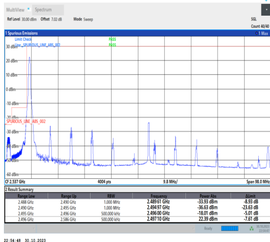
1-N41-30-90-L-1-DFT-PI2BPSK-Edge_1RB_Left-1@0-Ant1-1--PASS-see graph
