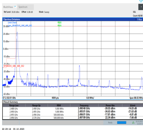
1-N41-30-80-L-4-CP-QPSK-Edge_1RB_Left-1@0-Ant1-1--PASS-see graph
