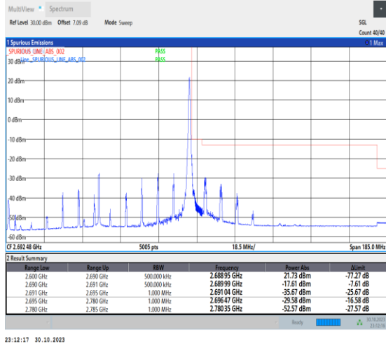
1-N41-30-90-H-2-DFT-PI2BPSK-Edge_1RB_Right-1@244-Ant1-1--PASS-see graph
