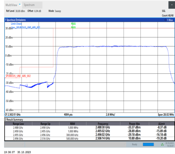
1-N41-30-20-L-3-DFT-PI2BPSK-Outer_Full-50@0-Ant1-1--PASS-see graph
