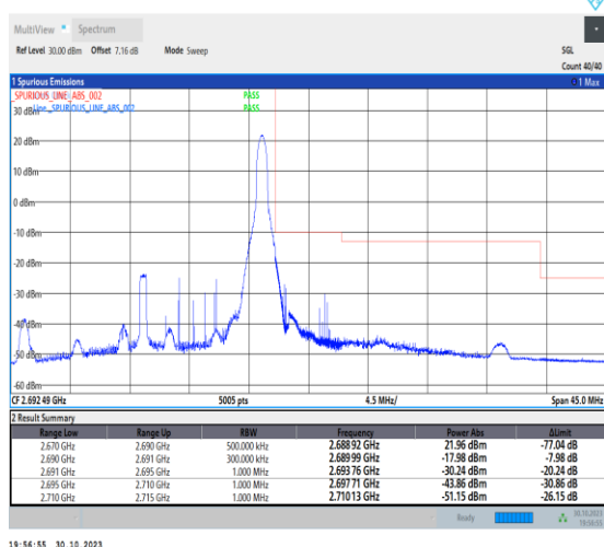
1-N41-30-20-H-5-CP-QPSK-Edge_1RB_Right-1@50-Ant1-1--PASS-see graph
