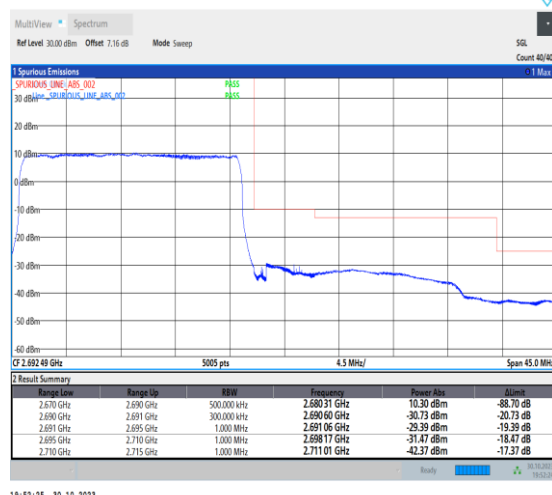
1-N41-30-20-H-3-DFT-PI2BPSK-Outer_Full-50@0-Ant1-1--PASS-see graph
