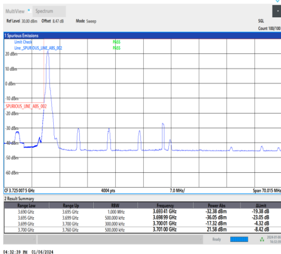
1-N77-3700-3980-30-60-L-4-CP-QPSK-Edge_1RB_Lef t-1@0-Ant2-1--PASS-see graph
