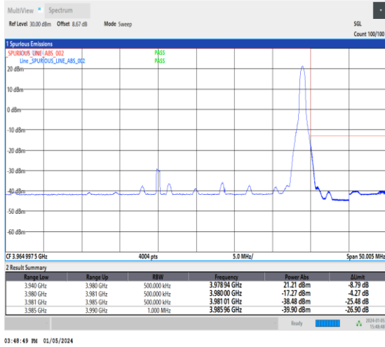
1-N77-3700-3980-30-40-H-2-DFT-PI2BPSK-Edge_1R B_Right-1@105-Ant2-1--PASS-see graph
