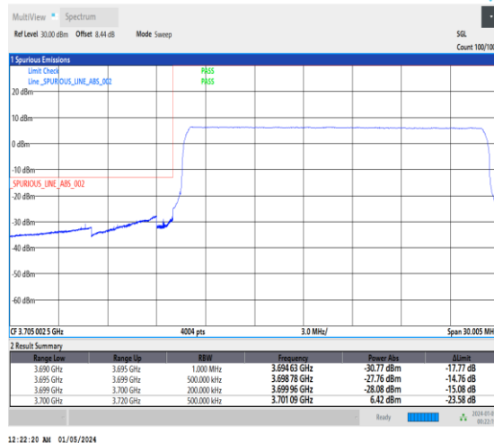
1-N77-3700-3980-30-20-L-6-CP-QPSK-Outer_Full -51@0-Ant2-1--PASS-see graph
