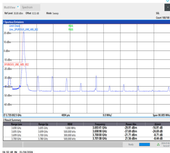
1-N77-3700-3980-30-80-L-1-DFT-PI2BPSK-Edge_1RB_Left-1@0-Ant2-1--PASS-see graph
