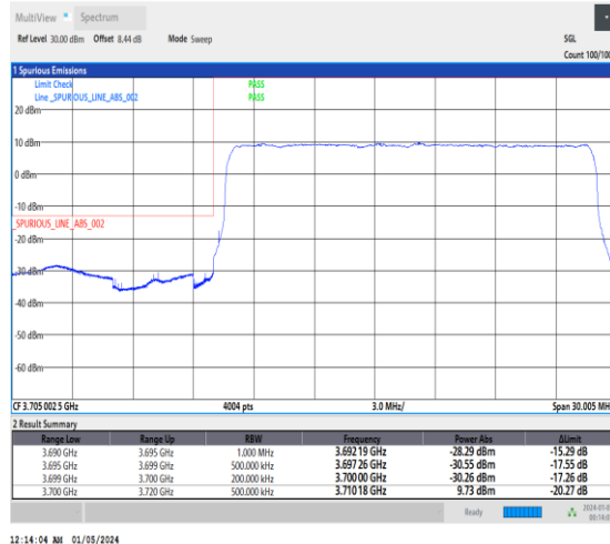
1-N77-3700-3980-30-20-L-3-DFT-PI2BPSK-Outer _Full-50@0-Ant2-1--PASS-see graph
