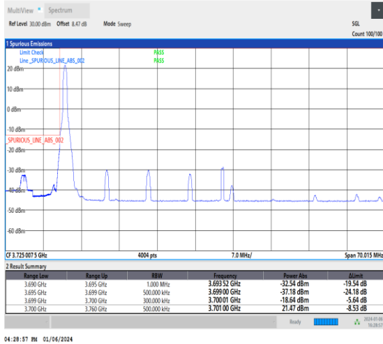
1-N77-3700-3980-30-60-L-1-DFT-PI2BPSK-Edge_1RB_Left-1@0-Ant2-1--PASS-see graph
