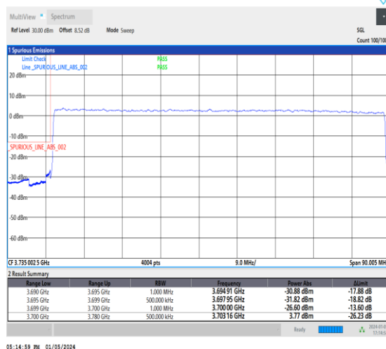
1-N77-3700-3980-30-80-L-3-DFT-PI2BPSK-Outer_Full-216@0-Ant2-1--PASS-see graph
