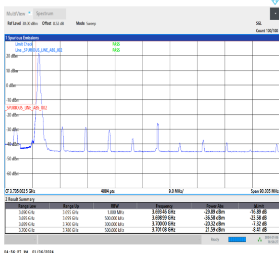
1-N77-3700-3980-30-80-L-4-CP-QPSK-Edge_1RB_Lef t-1@0-Ant2-1--PASS-see graph
