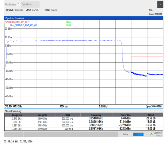
1-N77-3700-3980-30-40-H-3-DFT-PI2BPSK-Outer _Full-100@0-Ant2-1--PASS-see graph
