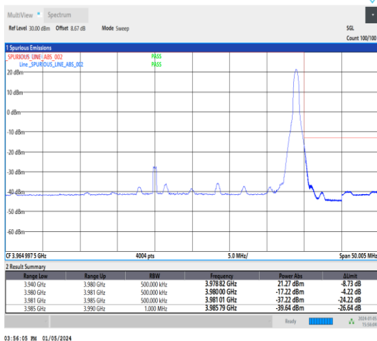
1-N77-3700-3980-30-40-H-5-CP-QPSK-Edge_1RB_Ri ght-1@105-Ant2-1--PASS-see graph
