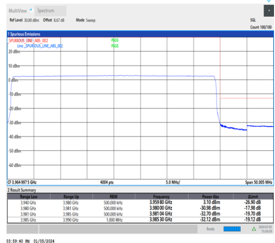
1-N77-3700-3980-30-40-H-6-CP-QPSK-Outer_Full -106@0-Ant2-1--PASS-see graph
