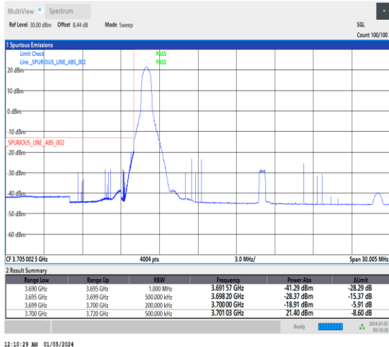
1-N77-3700-3980-30-20-L-1-DFT-PI2BPSK-Edge_1RB _Left-1@0-Ant2-1--PASS-see graph
