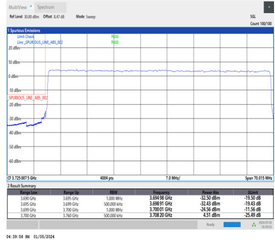
1-N77-3700-3980-30-60-L-3-DFT-PI2BPSK-Outer_Full-162@0-Ant2-1--PASS-see graph
