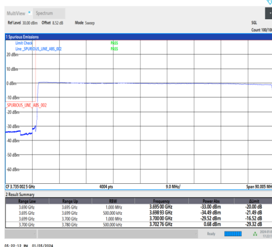
1-N77-3700-3980-30-80-L-6-CP-QPSK-Outer_Full -217@0-Ant2-1--PASS-see graph
