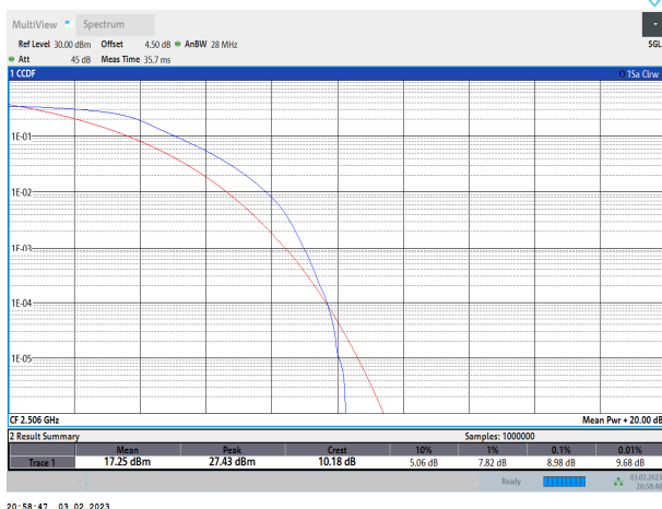
Band41-20MHz-QPSK-40620-100RB#0
