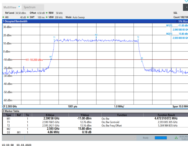
Band41-5MHz-QPSK-40620-25RB#0
