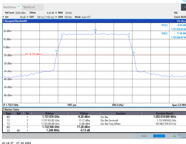
Band4-1.4MHz-QPSK-20175-6RB#0
