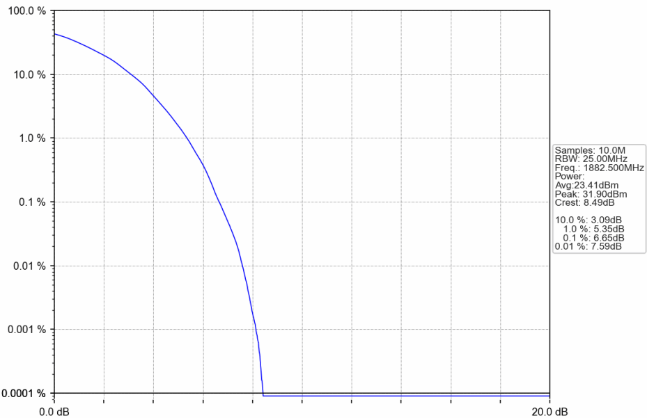
Band25 15MHz 64QAM MCH 1882.5MHz RB 75 0 NTNV
