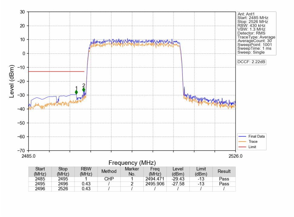
Band41 20MHz 16QAM LCH 2506MHz RB 100 0 NTNV
