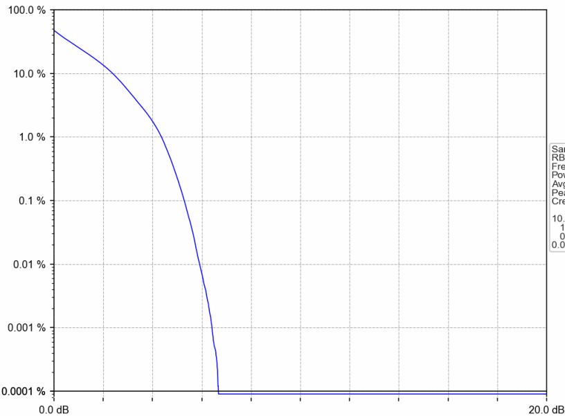
Band66_5MHz_QPSK_MCH_1745MHz_RB_25_0_NTNV
