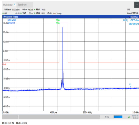
1-N25-15-40-H-1-DFT-PI2BPSK-Inner_1RB_Left-1@ 1-1000-3000-Ant1-2867.50--39.55--13-PASS
