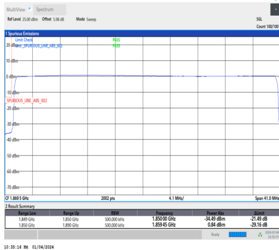
1-N25-15-40-L-6-CP-QPSK-Outer_Full-216@0-Ant1-1-seegraph-PASS-see graph
