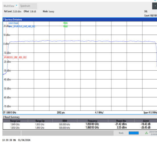
1-N25-15-40-L-3-DFT-PI2BPSK-Outer_Full-216@0-Ant1-1-seegraph-PASS-see graph
