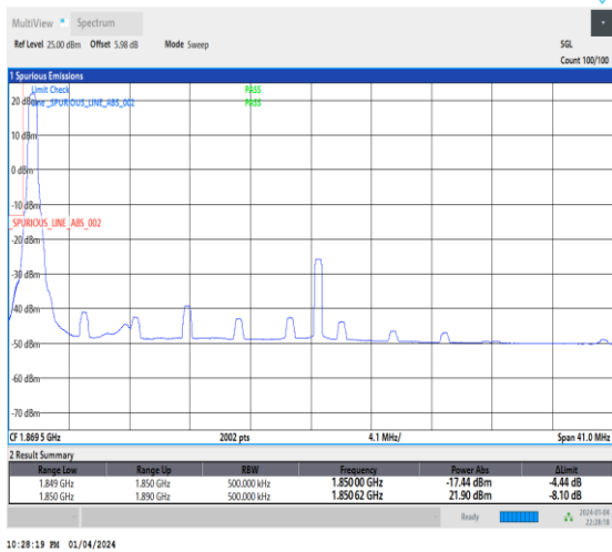
1-N25-15-40-L-1-DFT-PI2BPSK-Edge_1RB_Left-1@0-Ant1-1-seegraph-PASS-see graph
