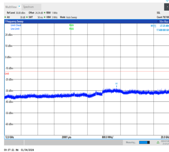
1-N25-15-40-H-1-DFT-PI2BPSK-Inner_1RB_Left-1@ 1-12000-20000-Ant1-17408.00--27.25--13-PASS
