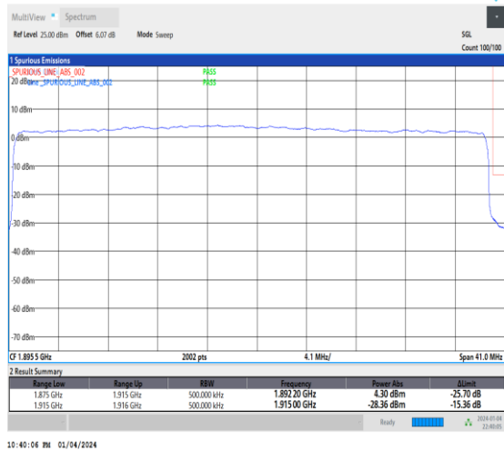
1-N25-15-40-H-3-DFT-PI2BPSK-Outer_Full-216@0-Ant1-1-seegraph-PASS-see graph
