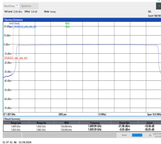
1-N25-15-15-L-6-CP-QPSK-Outer_Full-79@0-Ant1-1-seegraph-PASS-see graph
