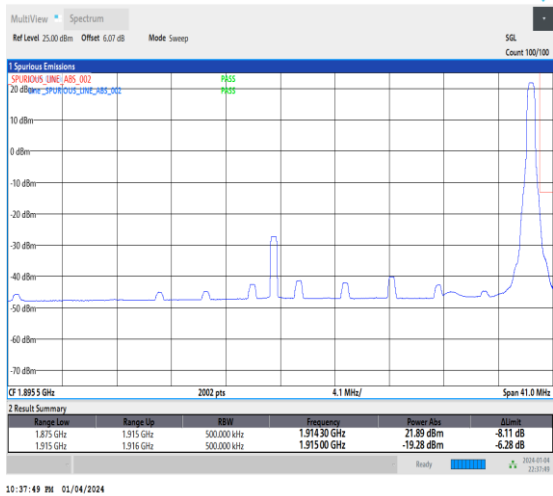
1-N25-15-40-H-2-DFT-PI2BPSK-Edge_1RB_Right-1@215-Ant1-1-seegraph-PASS-see graph
