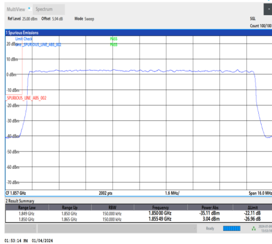
1-N25-15-15-L-3-DFT-PI2BPSK-Outer_Full-75@0-Ant1-1-seegraph-PASS-see graph
