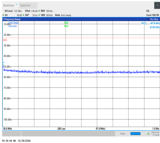
1-N25-15-40-H-1-DFT-PI2BPSK-Inner_1RB_Left-1 @1-30-1000-Ant1-35.34--49.78--23-PASS
