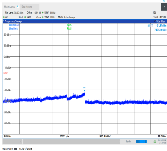
1-N25-15-40-H-1-DFT-PI2BPSK-Inner_1RB_Left-1 @ 1-3000-12000-Ant1-7471.20--31.34--13-PASS
