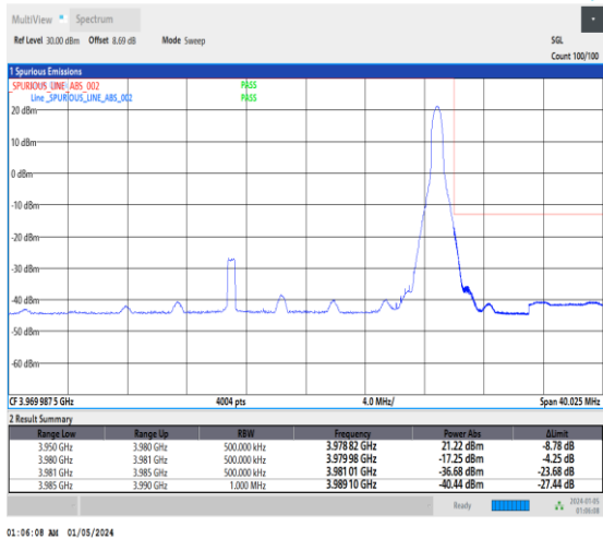
1-N77-3700-3980-30-30-H-5-CP-QPSK-Edge_1RB_Ri ght-1@77-Ant2-1--PASS-see graph
