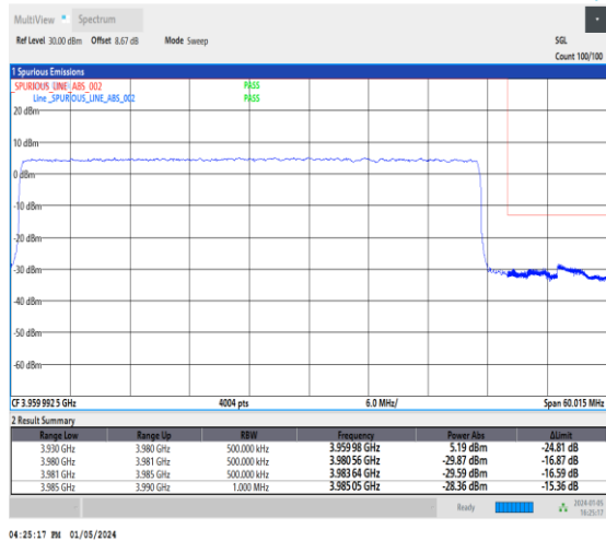
1-N77-3700-3980-30-50-H-3-DFT-PI2BPSK-Outer _Full-128@0-Ant2-1--PASS-see graph
