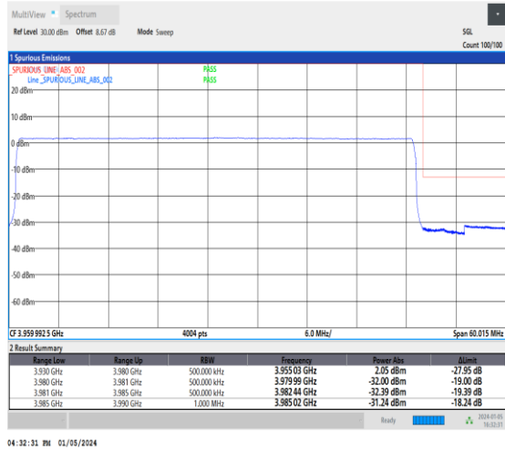
1-N77-3700-3980-30-50-H-6-CP-QPSK-Outer_Full -133@0-Ant2-1--PASS-see graph
