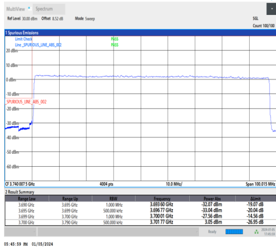
1-N77-3700-3980-30-90-L-3-DFT-PI2BPSK-Outer _Full-240@0-Ant2-1--PASS-see graph
