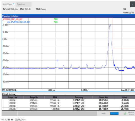
1-N77-3700-3980-30-50-H-2-DFT-PI2BPSK-Edge_1R B_Right-1@132-Ant2-1--PASS-see graph
