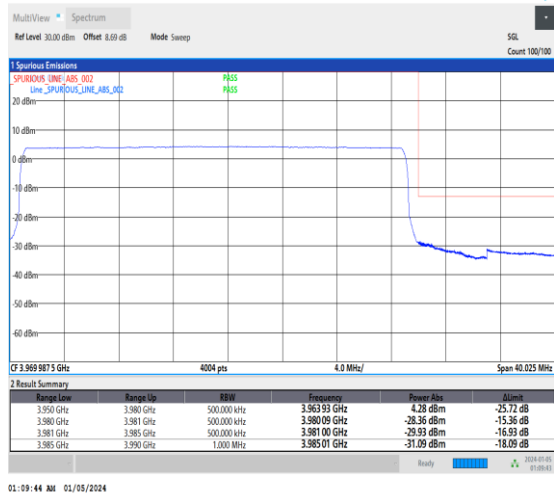
1-N77-3700-3980-30-30-H-6-CP-QPSK-Outer_Full -78@0-Ant2-1--PASS-see graph
