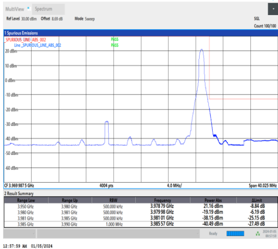
1-N77-3700-3980-30-30-H-2-DFT-PI2BPSK-Edge_1R B_Right-1@77-Ant2-1--PASS-see graph
