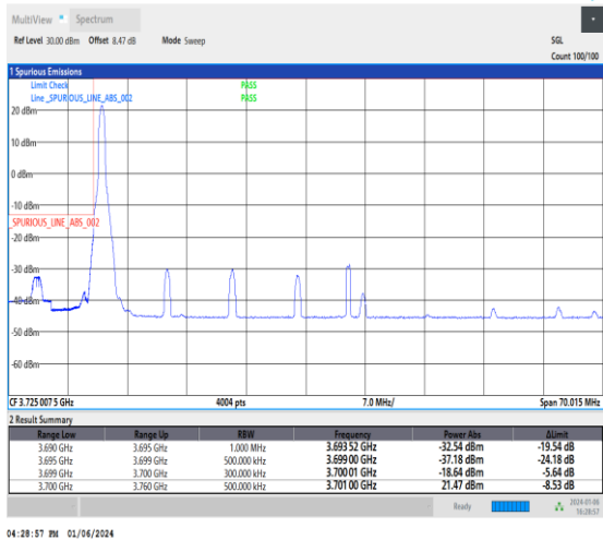
1-N77-3700-3980-30-60-L-1-DFT-PI2BPSK-Edge_1RB_Left-1@0-Ant2-1--PASS-see graph
