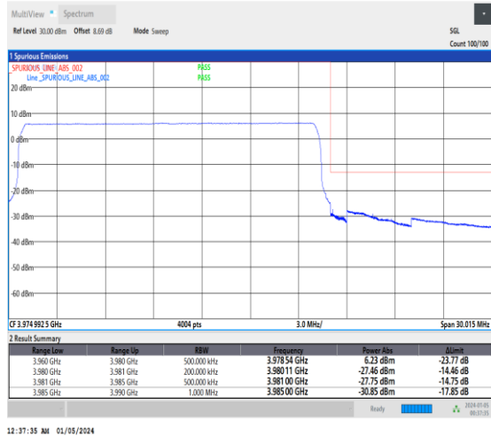
1-N77-3700-3980-30-20-H-6-CP-QPSK-Outer_Full -51@0-Ant2-1--PASS-see graph
