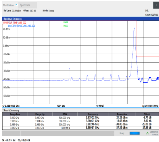
1-N77-3700-3980-30-60-H-5-CP-QPSK-Edge_1RB_Ri ght-1@161-Ant2-1--PASS-see graph
