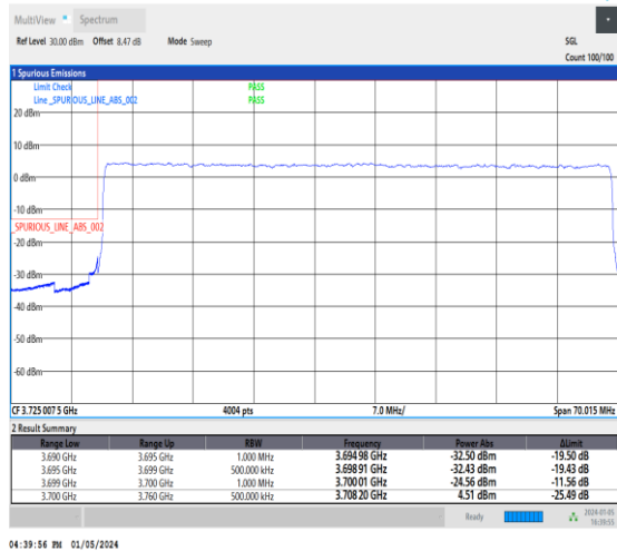
1-N77-3700-3980-30-60-L-3-DFT-PI2BPSK-Outer_Full-162@0-Ant2-1--PASS-see graph
