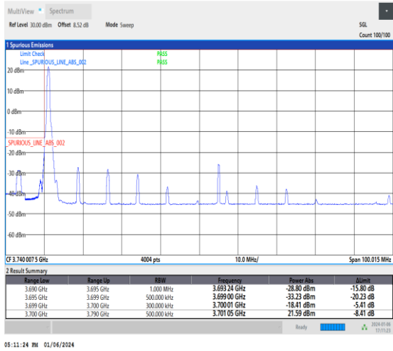
1-N77-3700-3980-30-90-L-4-CP-QPSK-Edge_1RB_Lef t-1@0-Ant2-1--PASS-see graph
