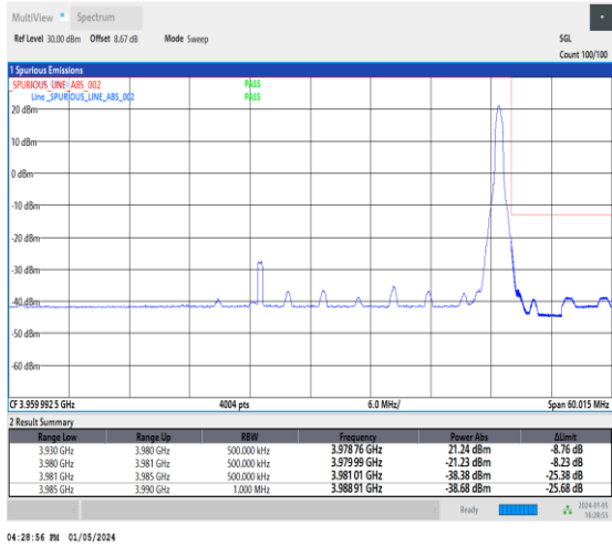
1-N77-3700-3980-30-50-H-5-CP-QPSK-Edge_1RB_Ri ght-1@132-Ant2-1--PASS-see graph
