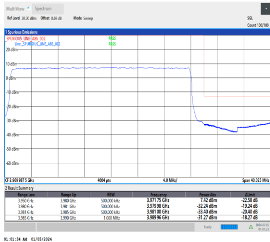
1-N77-3700-3980-30-30-H-3-DFT-PI2BPSK-Outer _Full-75@0-Ant2-1--PASS-see graph
