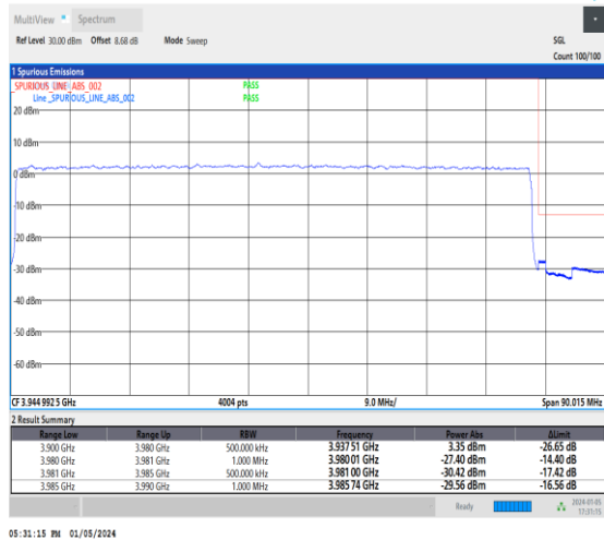
1-N77-3700-3980-30-80-H-3-DFT-PI2BPSK-Outer _Full-216@0-Ant2-1--PASS-see graph
