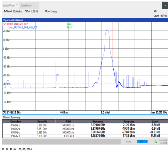
1-N77-3700-3980-30-20-H-2-DFT-PI2BPSK-Edge_1R B_Right-1@50-Ant2-1--PASS-see graph
