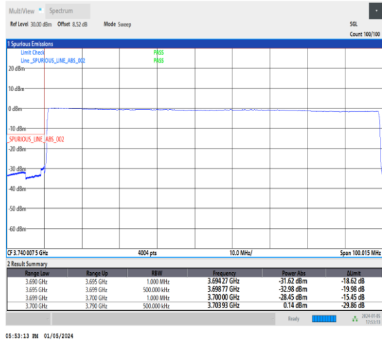
1-N77-3700-3980-30-90-L-6-CP-QPSK-Outer_Full -245@0-Ant2-1--PASS-see graph
