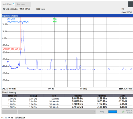
1-N77-3700-3980-30-60-L-4-CP-QPSK-Edge_1RB_Lef t-1@0-Ant2-1--PASS-see graph
