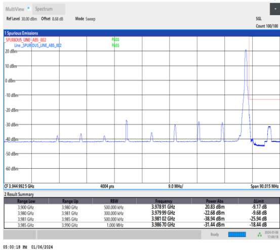
1-N77-3700-3980-30-80-H-2-DFT-PI2BPSK-Edge_1R B_Right-1@216-Ant2-1--PASS-see graph
