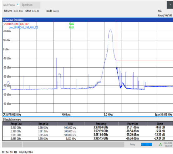
1-N77-3700-3980-30-20-H-5-CP-QPSK-Edge_1RB_Ri ght-1@50-Ant2-1--PASS-see graph
