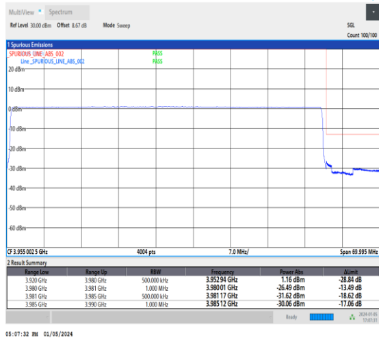
1-N77-3700-3980-30-60-H-6-CP-QPSK-Outer_Full -162@0-Ant2-1--PASS-see graph
