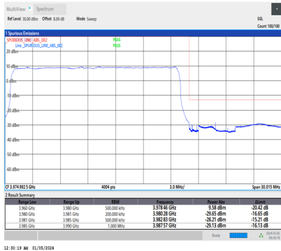
1-N77-3700-3980-30-20-H-3-DFT-PI2BPSK-Outer _Full-50@0-Ant2-1--PASS-see graph
