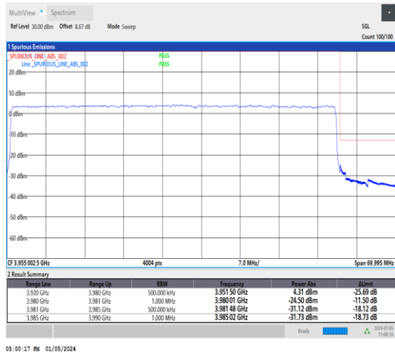
1-N77-3700-3980-30-60-H-3-DFT-PI2BPSK-Outer _Full-162@0-Ant2-1--PASS-see graph
