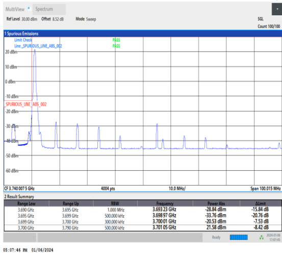
1-N77-3700-3980-30-90-L-1-DFT-PI2BPSK-Edge_1RB _Left-1@0-Ant2-1--PASS-see graph
