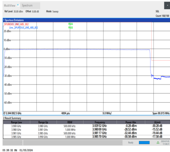
1-N77-3700-3980-30-80-H-6-CP-QPSK-Outer_Full -217@0-Ant2-1--PASS-see graph
