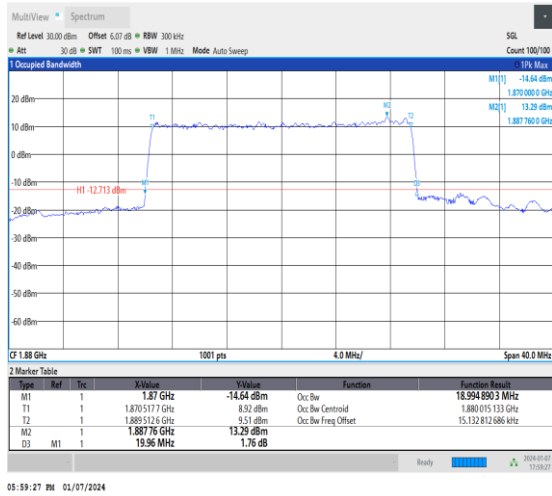
1-DC_5A_n2A-15-20-M-6-CP-QPSK-Outer_Full-106 @0-Ant1-18.995-19.960-≤20-PASS
