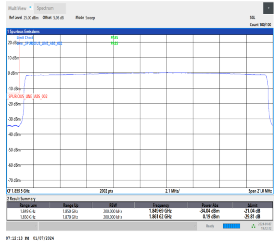
1-DC_5A_n2A-15-20-L-6-CP-QPSK-Outer_Full-106@0-Ant1-1-seegraph-PASS-see graph
