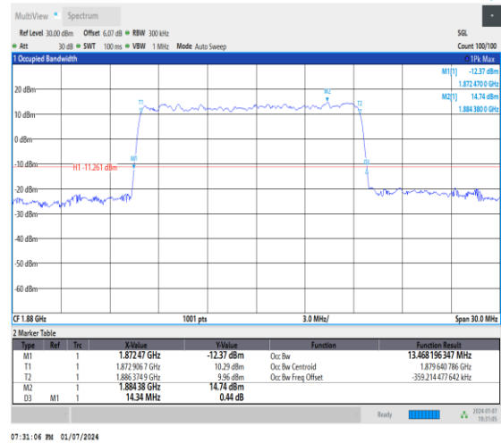
1-DC_5A_n2A-15-15-M-6-CP-QPSK-Outer_Full-79 @0-Ant1-13.468-14.34≤15-PASS
