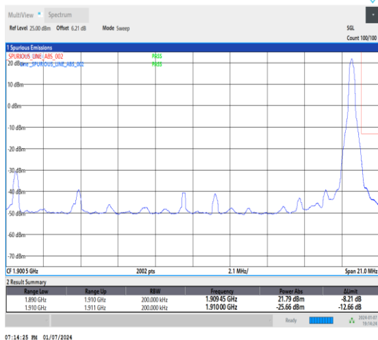
1-DC_5A_n2A-15-20-H-2-DFT-PI2BPSK-Edge_1RB_Left-1@0-Ant1-1-seegraph-PASS-see graph
