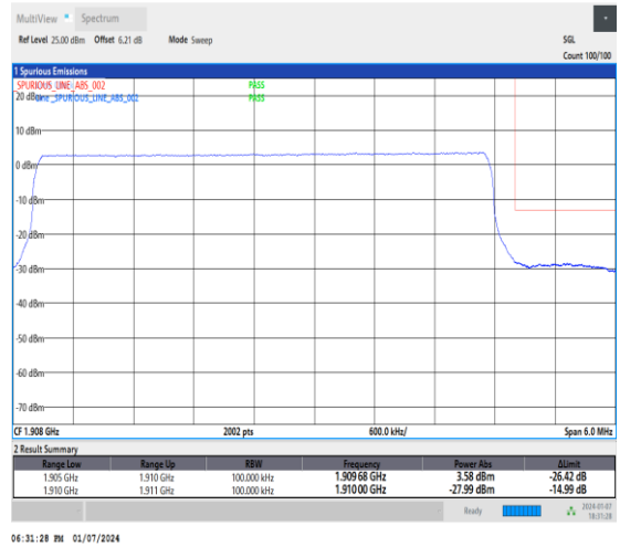
1-DC_5A_n2A-15-5-H-6-CP-QPSK-Outer_Full-25@0-Ant1-1-seegraph-PASS-see graph
