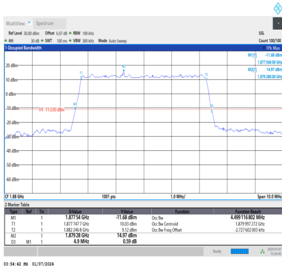
1-DC_5A_n2A-15-5-M-3-DFT-16QAM-Outer_Full-25 @0-Ant1-4.499-4.900≤5-PASS
