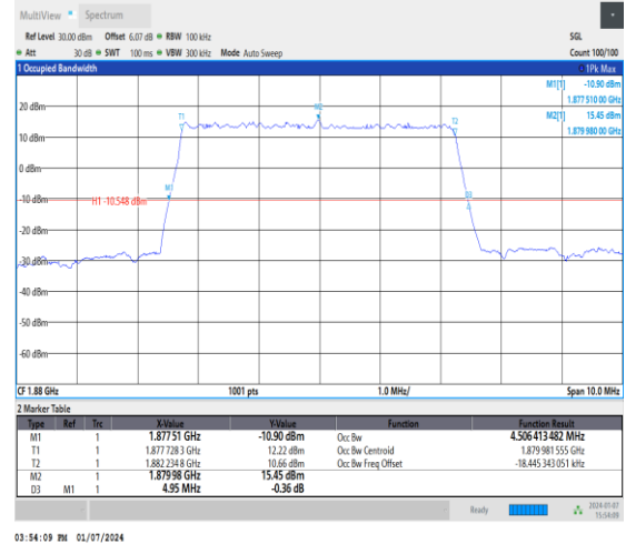
1-DC_5A_n2A-15-5-M-2-DFT-PI2BPSK-Outer_Full-2 5@0-Ant1-4.506-4.950-≤5-PASS
