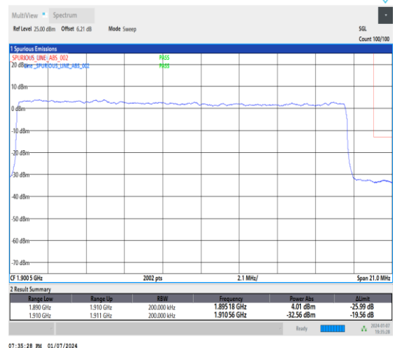
1-DC_5A_n2A-15-20-H-3-DFT-PI2BPSK-Outer_Full-106@0-Ant1-1-seegraph-PASS-see graph
