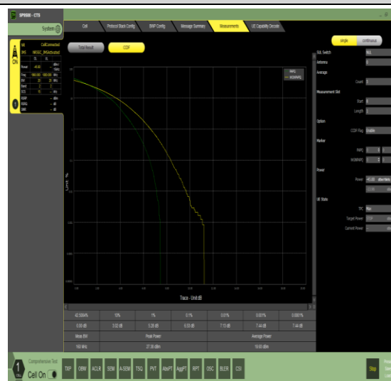
1-DC_5A_n2A-15-20-M-15-NS_01-CP-256QAM-Out er_Full-100@0-6.53
