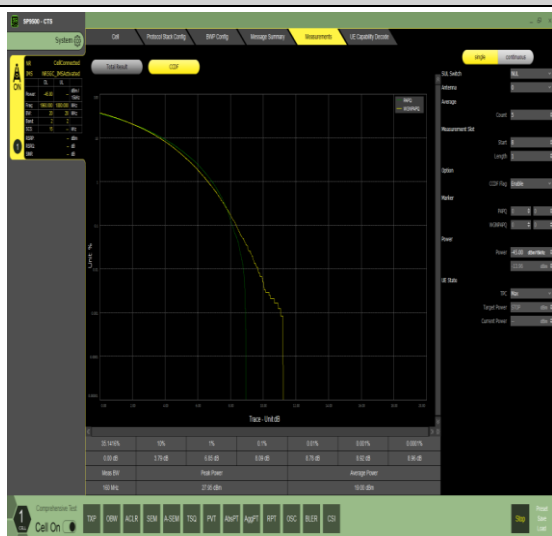
1-DC_5A_n2A-15-20-M-15-NS_01-DFT-256QAM-Out er_Full-100@0-8.09
