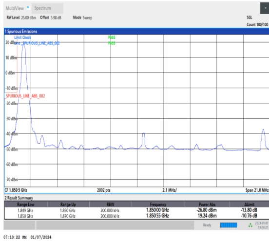
1-DC_5A_n2A-15-20-L-4-CP-QPSK-Edge_1RB_Left-1@0-Ant1-1-seegraph-PASS-see graph
