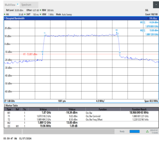
1-DC_5A_n2A-15-20-M-7-CP-16QAM-Outer_Full-10 6@0-Ant1-18.966-19.960-≤20-PASS
