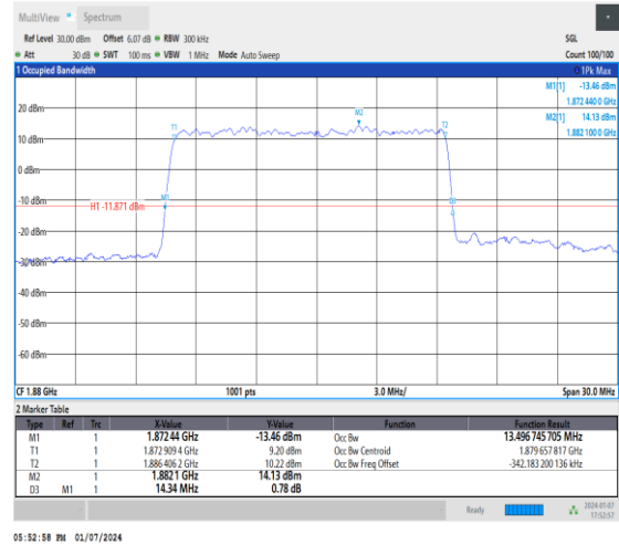
1-DC_5A_n2A-15-15-M-4-DFT-64QAM-Outer_Full-7 5@0-Ant1-13.497-14.340≤15-PASS
