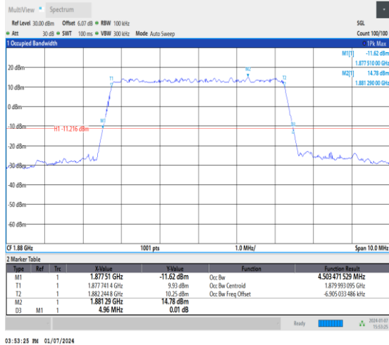
1-DC_5A_n2A-15-5-M-1-DFT-QPSK-Outer_Full-25 @0-Ant1-4.503-4.960-≤5-PASS
