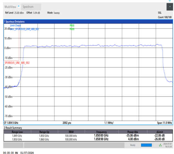
1-DC_5A_n2A-15-10-L-3-DFT-PI2BPSK-Outer_Ful
