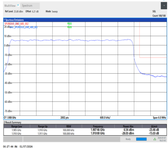
1-DC_5A_n2A-15-5-H-3-DFT-PI2BPSK-Outer_Full-25@0-Ant1-1-seegraph-PASS-see graph
