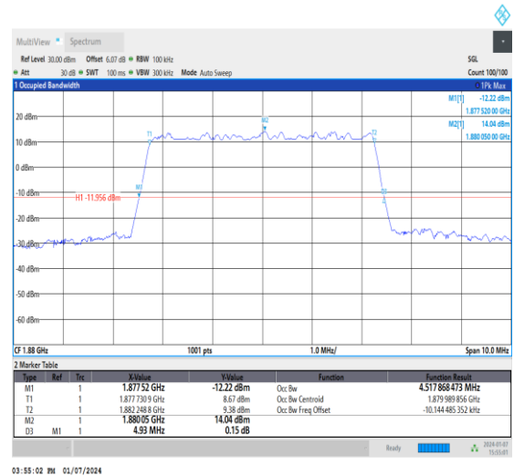
1-DC_5A_n2A-15-5-M-4-DFT-64QAM-Outer_Full-25 @0-Ant1-4.518-4.930-≤5-PASS
