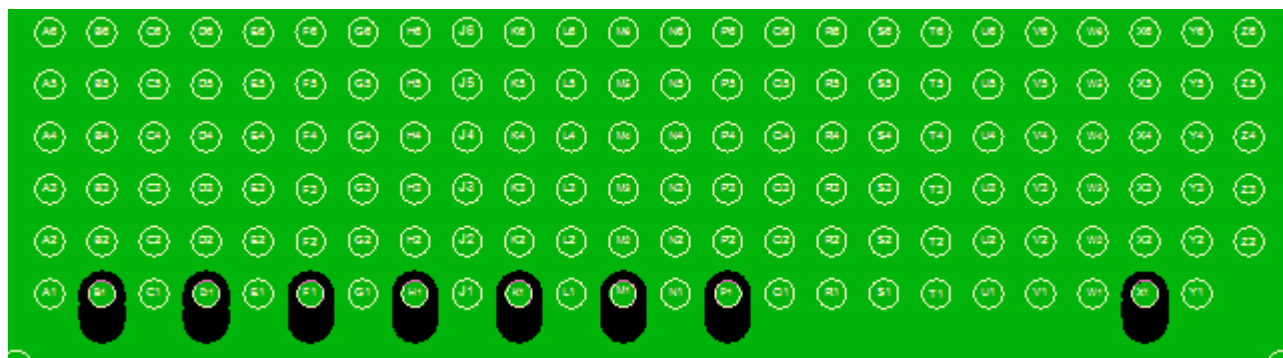
Figure 9-1: Antenna Pad Ground Cutouts (NAD bottom layer)
