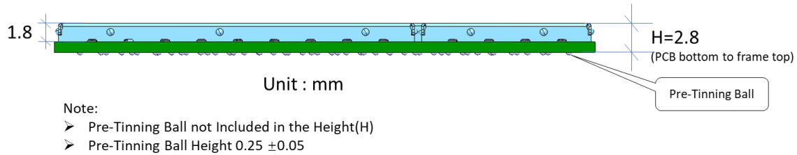
Figure 6-3 Module Side View
