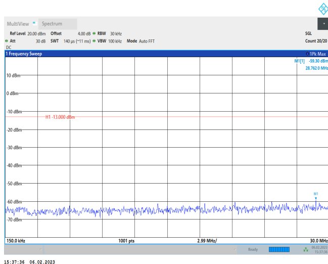
Band V-4132-0.15~30MHz
