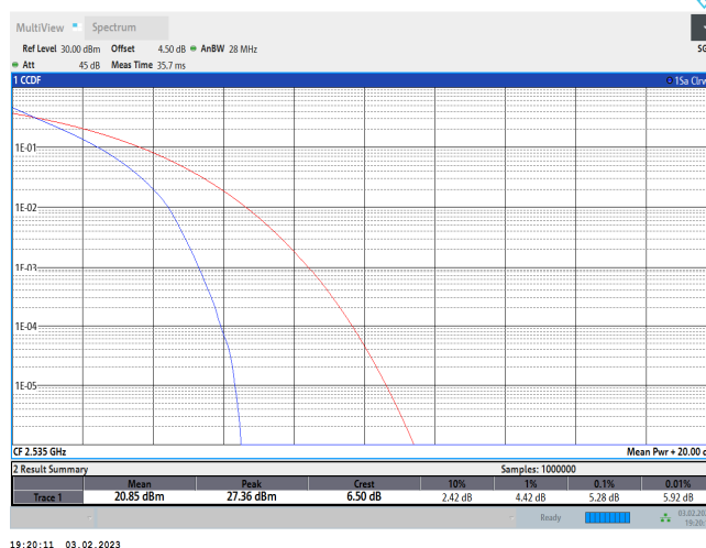
Band7-20MHz-QPSK-21100-100RB#0
