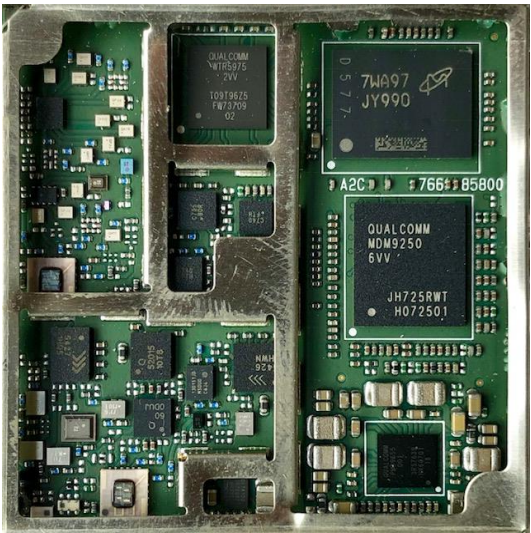
Fig. 2. WT50NA01 top view with the shield removed.
