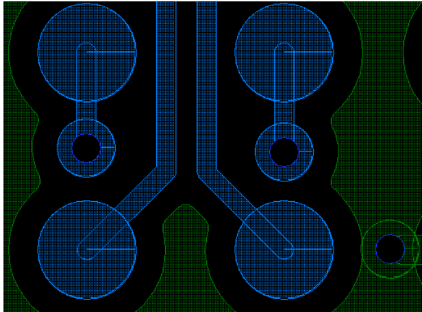
Figure 1 Vias placed between Pads
