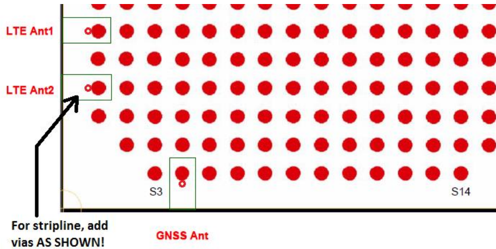
Figure 3: Antenna Pad Ground Cutout (Top View)
