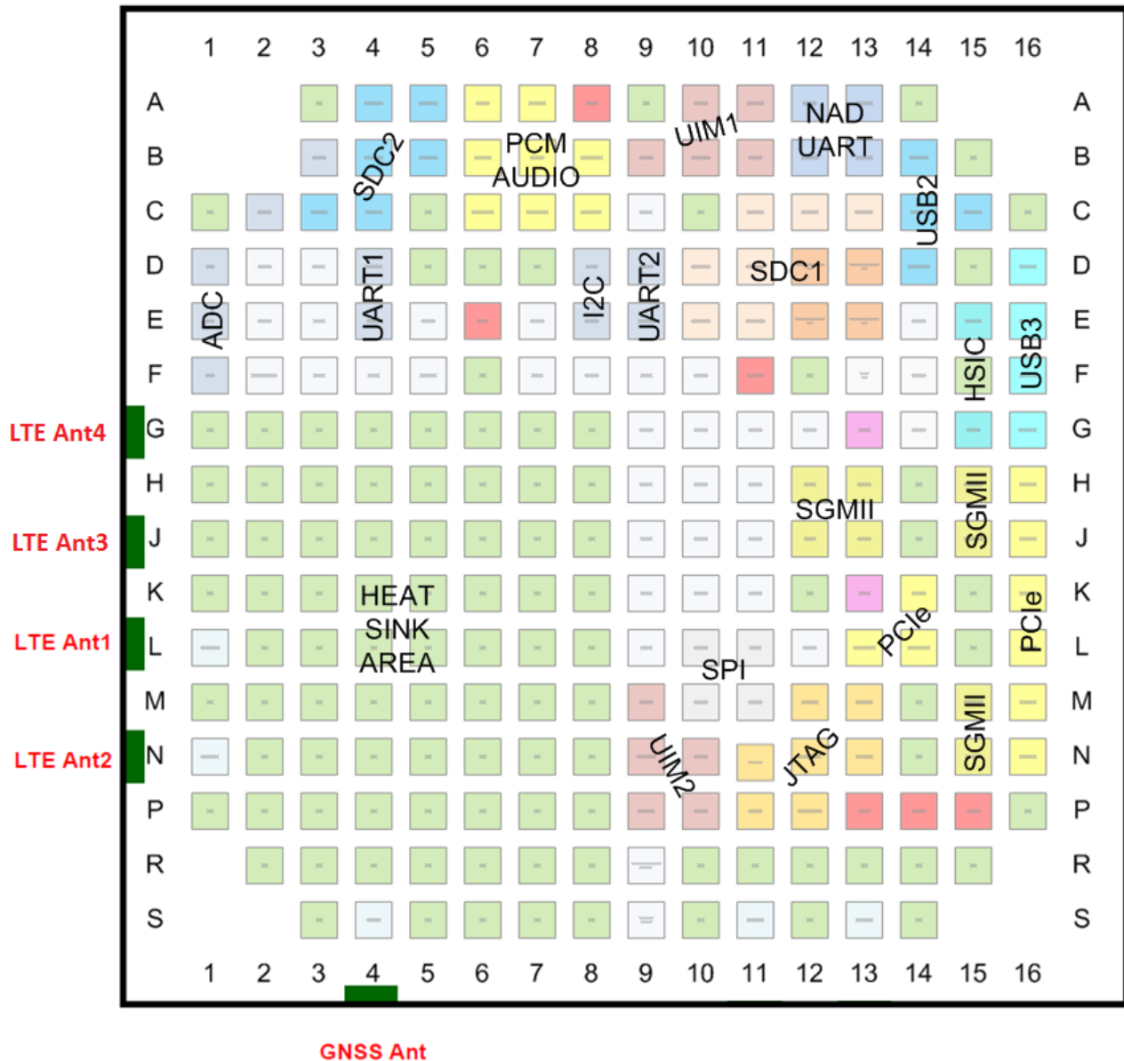
Figure 2: NAD Pin Breakout
