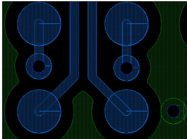
Figure 1 Vias placed between Pads
