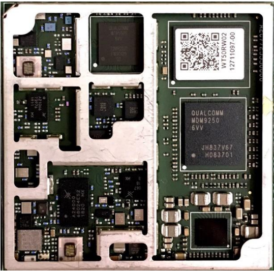
Fig. 2. WT50RW02 top view with the shield removed.
