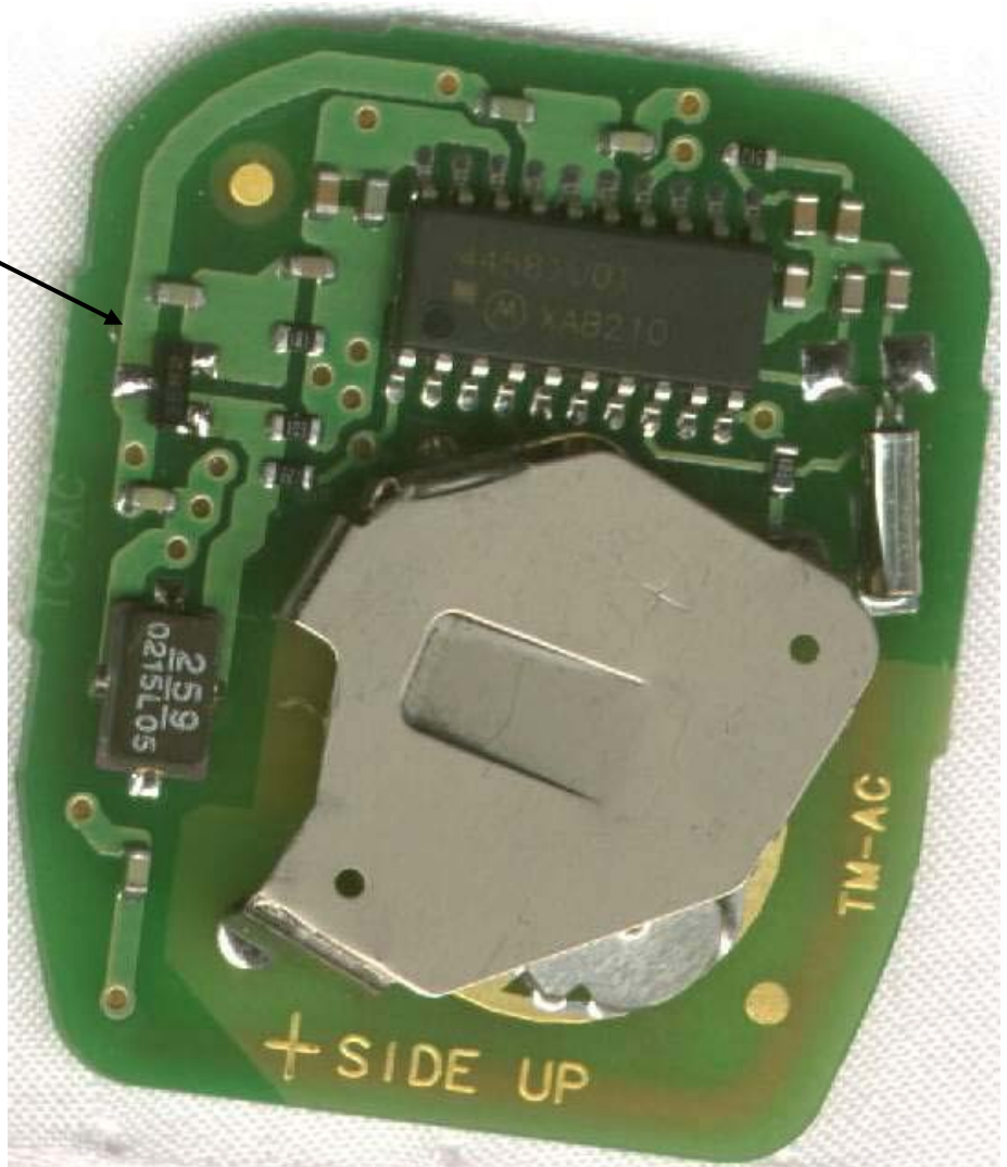
Photograph of Front of Circuit Board
