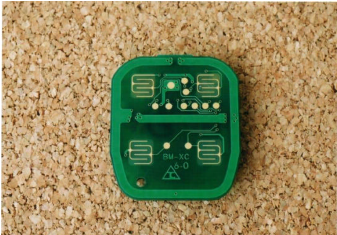
LHJ011 Transmitter PCB - Bottom
