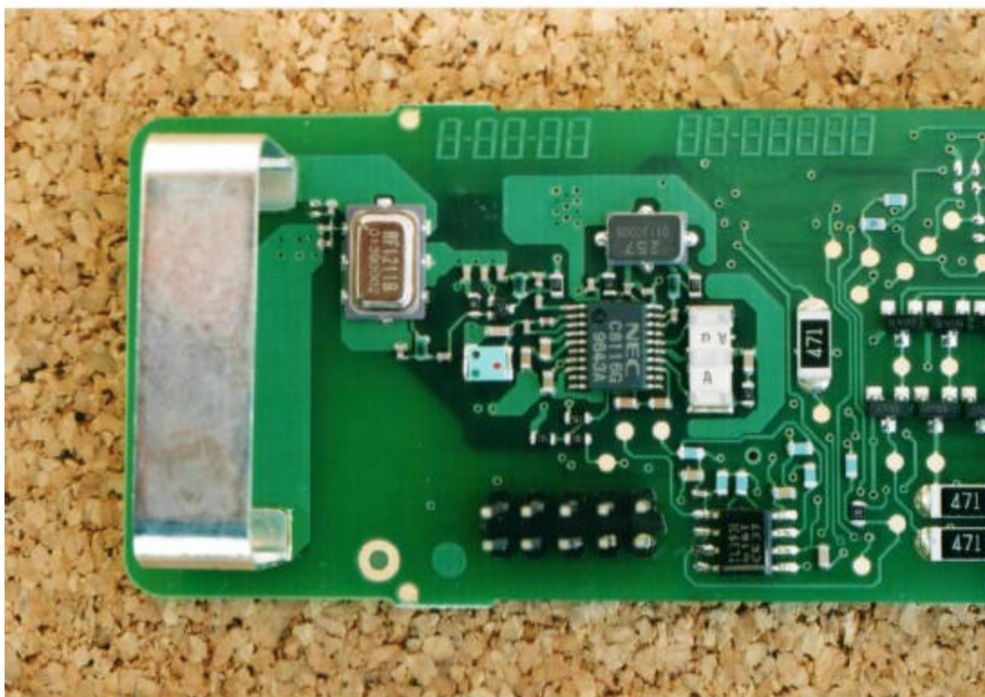
LHJ012 Receiver PCB RF Section Close-up Top
