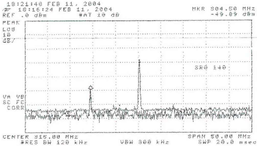
Figure 6.1. Relative receiver emissions with and without 315 MHz RF source.
