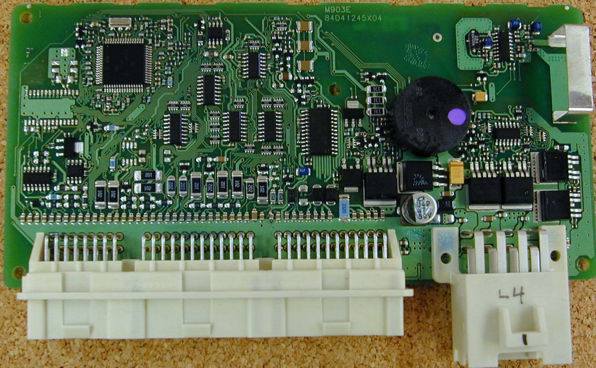
L4, PCB top
