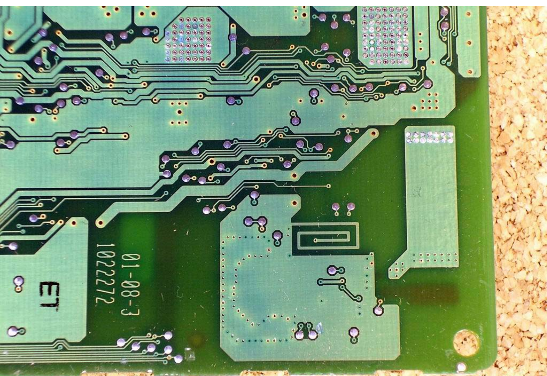
PCB (RF Section Close-up - bottom)
