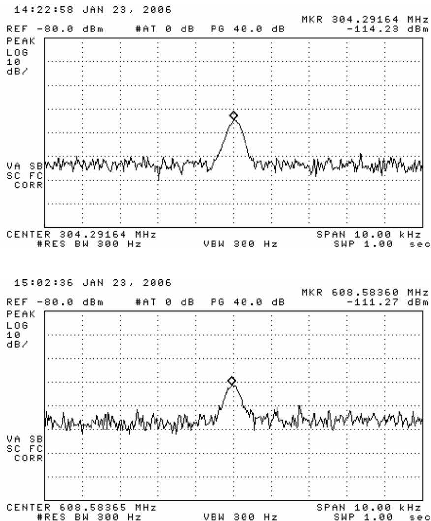
Figure 6.1. Relative receiver emissions.
