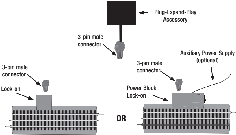
Figure 1. Plug-Expand-Play wiring
