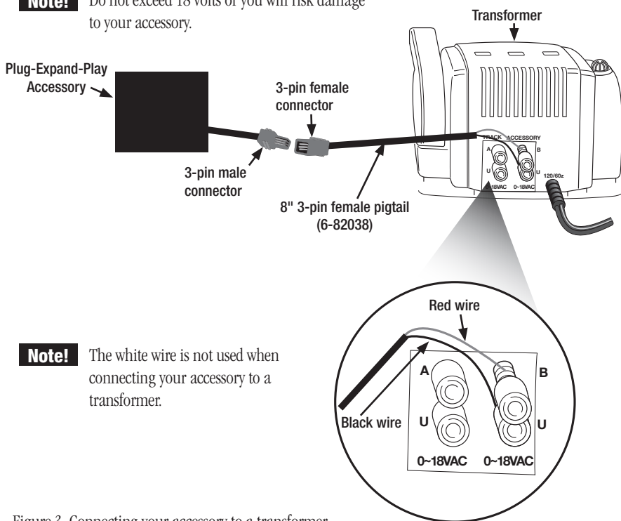
Figure 3. Connecting your accessory to a transformer.
