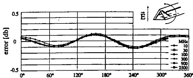
Fig. 6. Deviation from isotropy of the probe with triangular design in air, whereby the E-field was rotated in a plane normal to the probe axis. Measured using the TEM cell (if1110) between 10 MHz and 900 MHz and the waveguide R26 at 2500 MHz.
