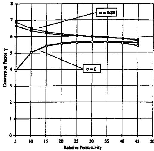
Fig. 12. Simulation: conversion factor at 900 MHz as a function of the relative permittivity of the biological tissue. Done for absorbing biological tissue and nonabsorbing tissue. MAFIA modeling are displayed by squares, MMP modeling by circles.
