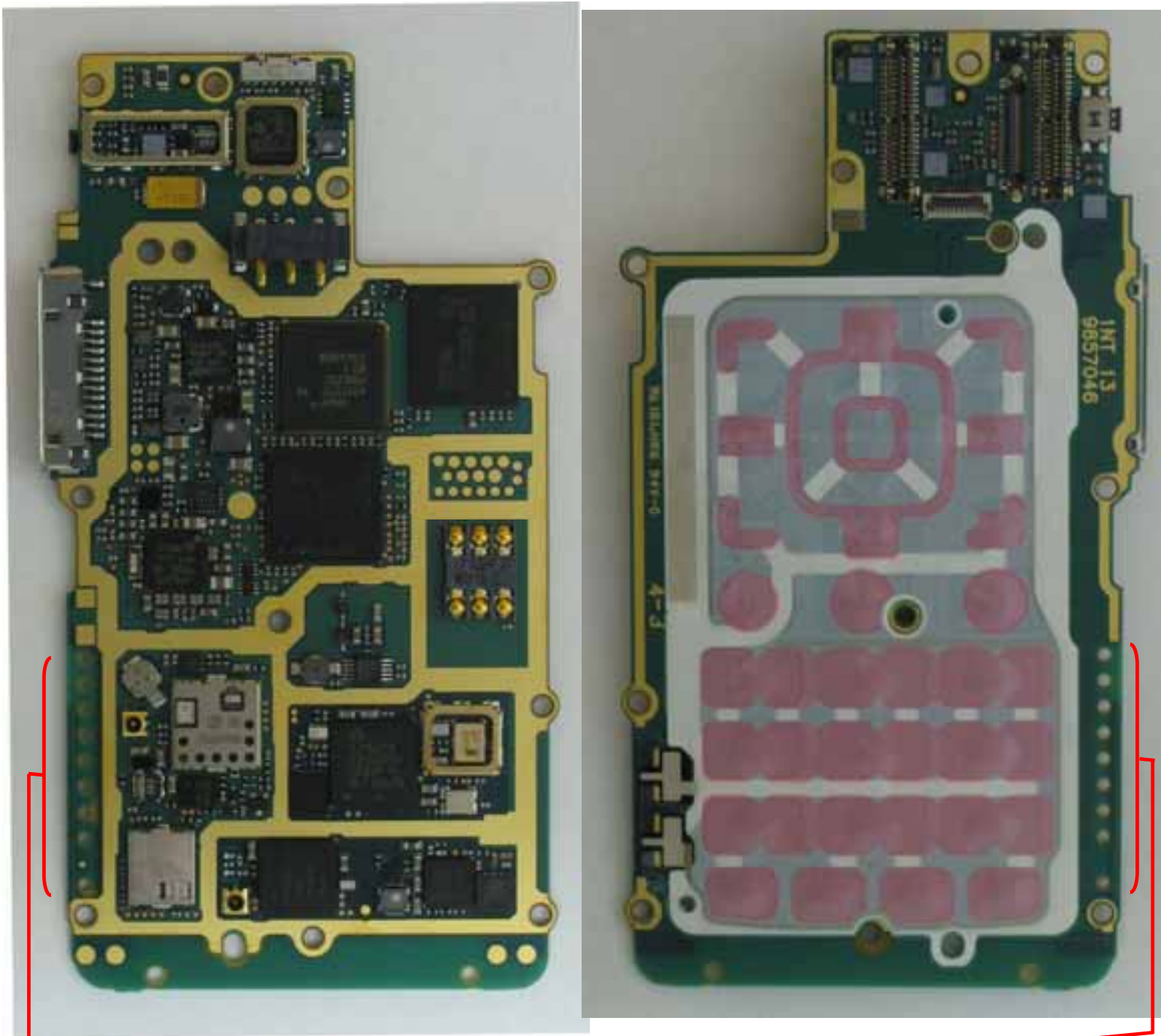
WLAN/BT Antenna
