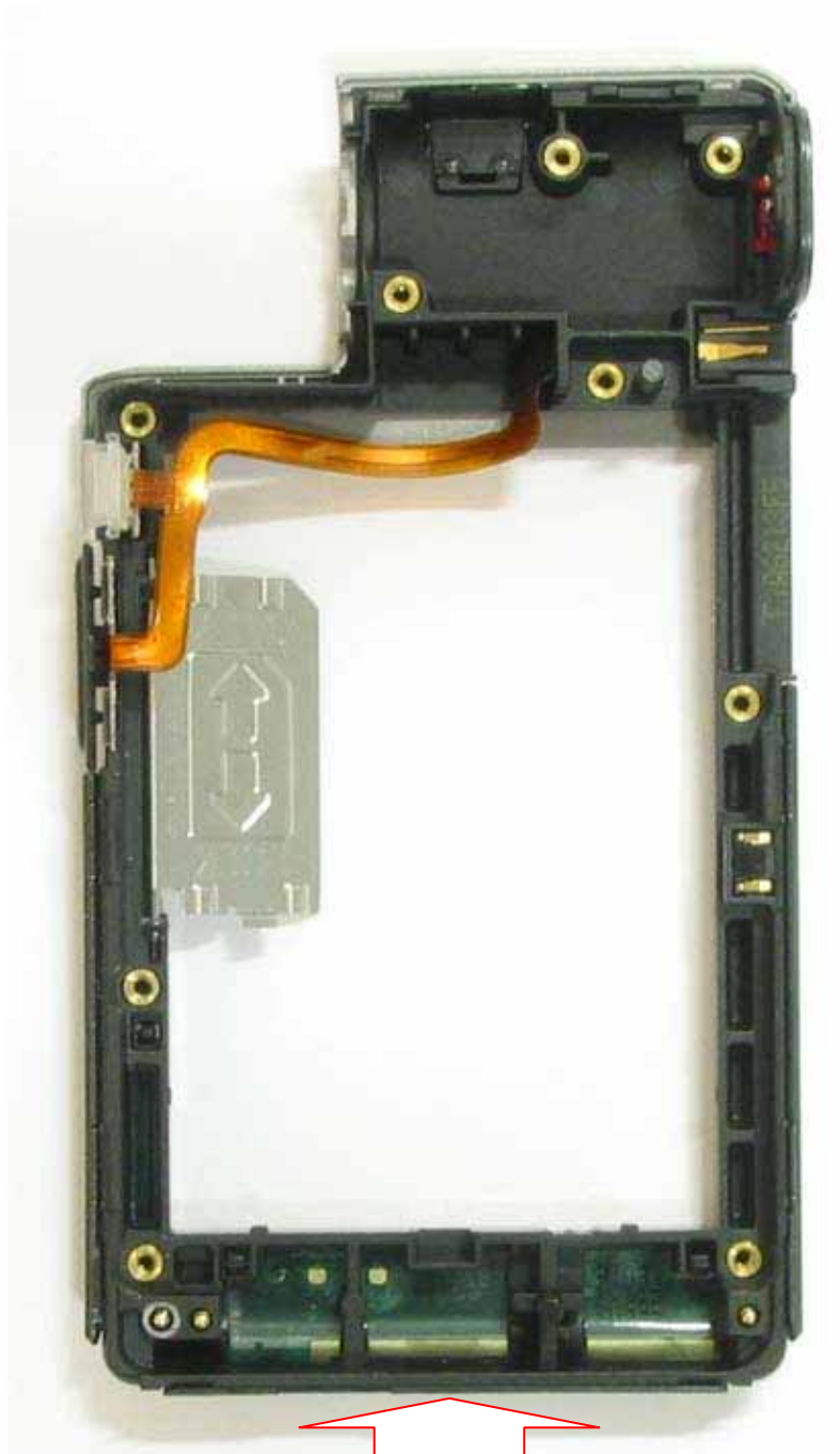
Cellular Antenna
