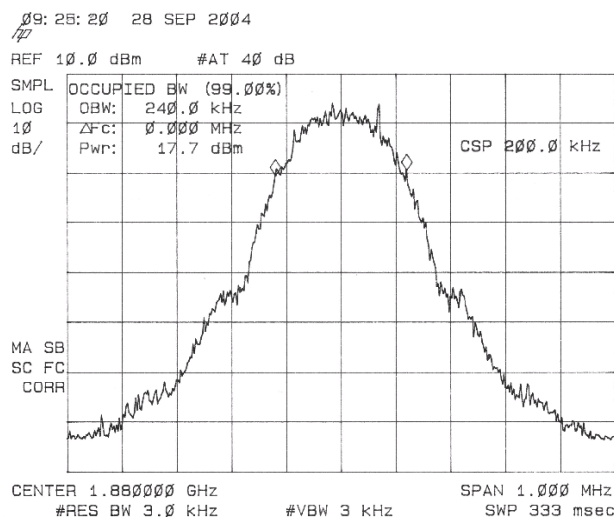
Picture 4. 99% occupied bandwidth GSM, channel 661
