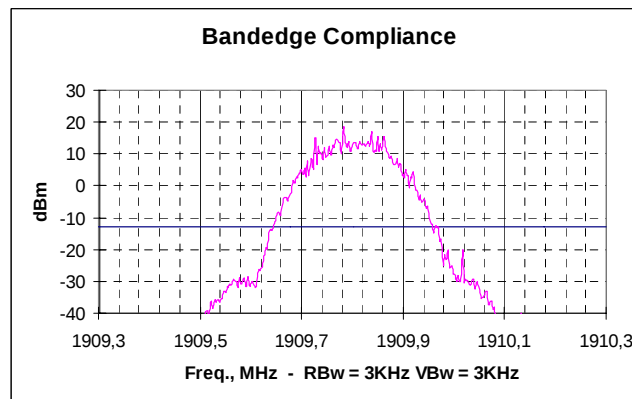
Picture 9. Upper bandedge, EGPRS channel 810
