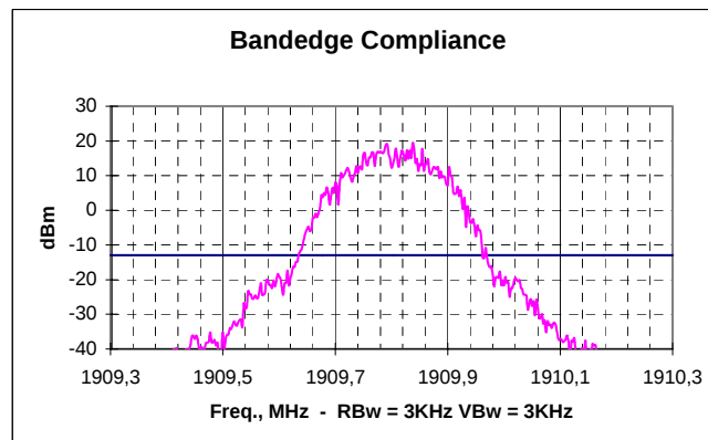
Picture 7. Upper bandedge, GSM channel 810
