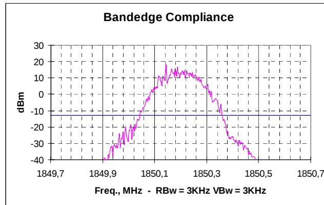
Picture 8. Lower bandedge, EGPRS channel 512
