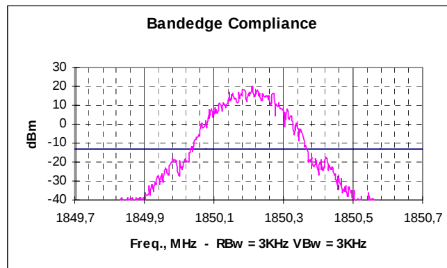
Picture 6. Lower bandedge, GSM channel 512
