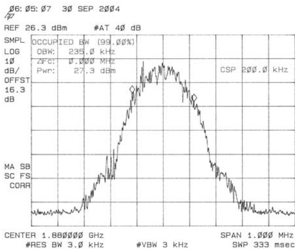
Picture 5. 99% occupied bandwidth EGRPS, channel 661
