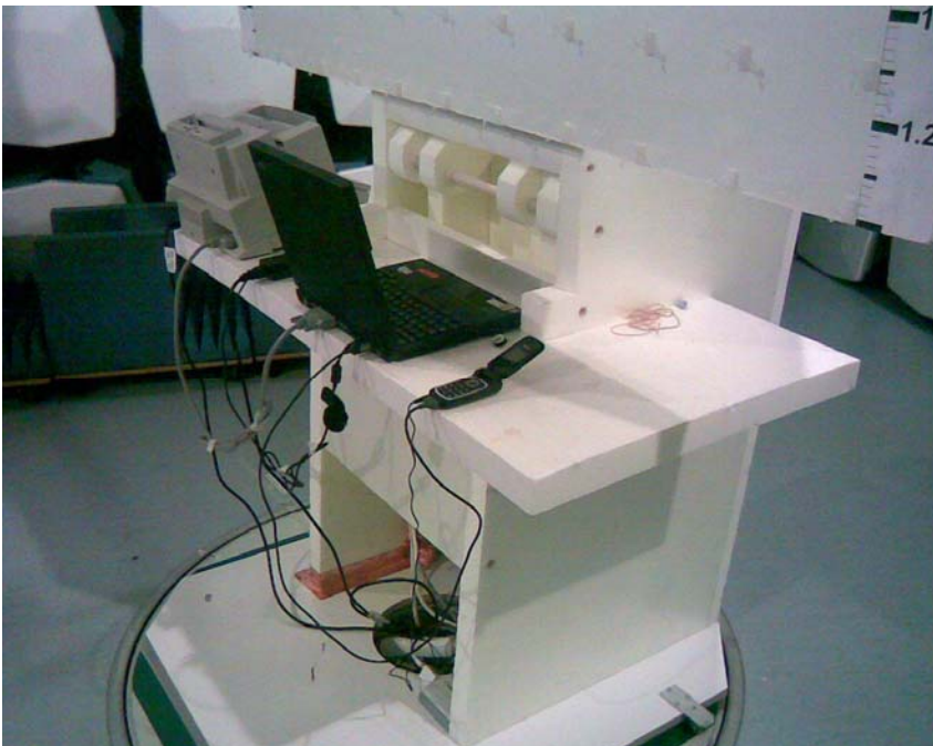
Picture 2 Radiated emission measurement GSM RX/Bluetooth TX + Computer peripherals
