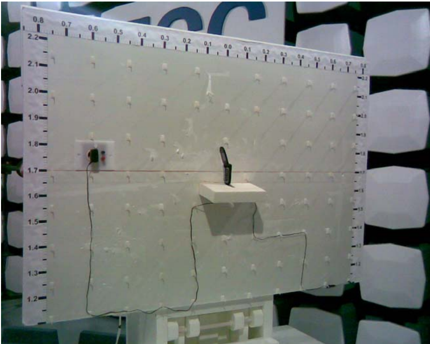
Picture 1 Spurious radiated emission measurement
