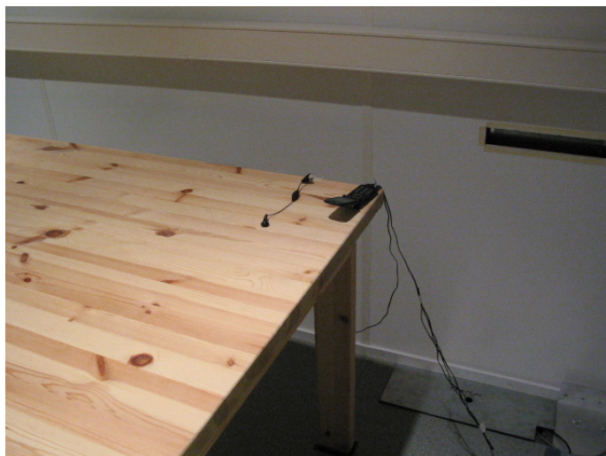
Picture 2 AC powerline conducted emission measurement WLAN TX
