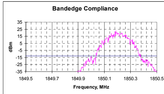
Lower bandedge, channel 512 GSM RBw = VBw = 3KHz
