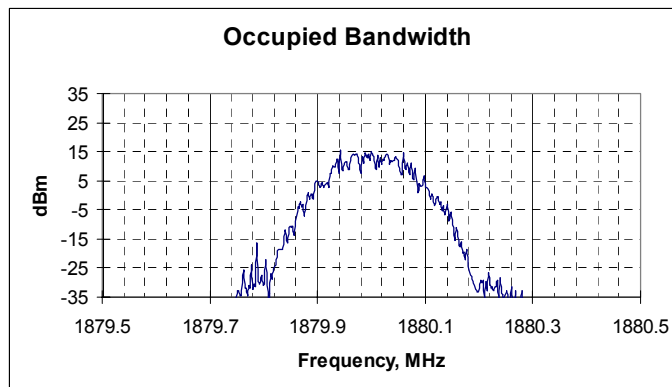
Picture 5. 99% occupied bandwidth, channel 661 EGPRS1900
