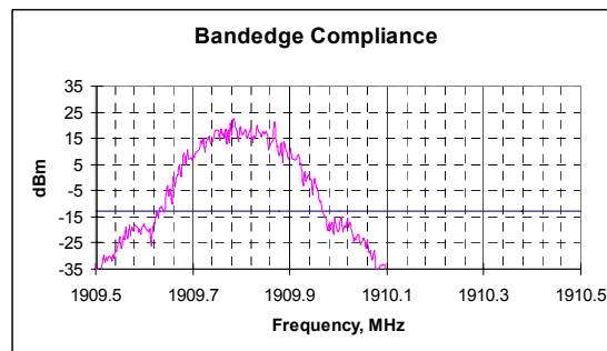
Upper bandedge, channel 810 GSM RBw = VBw = 3KHz
