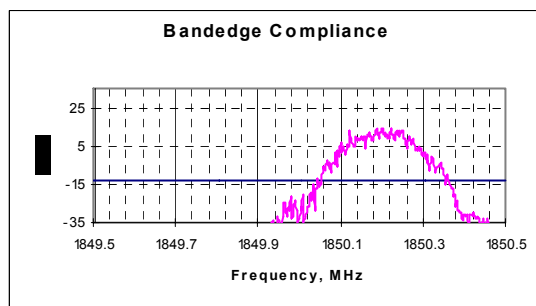
Lower bandedge, channel 512 EGPRS RBw = VBw = 3KHz
