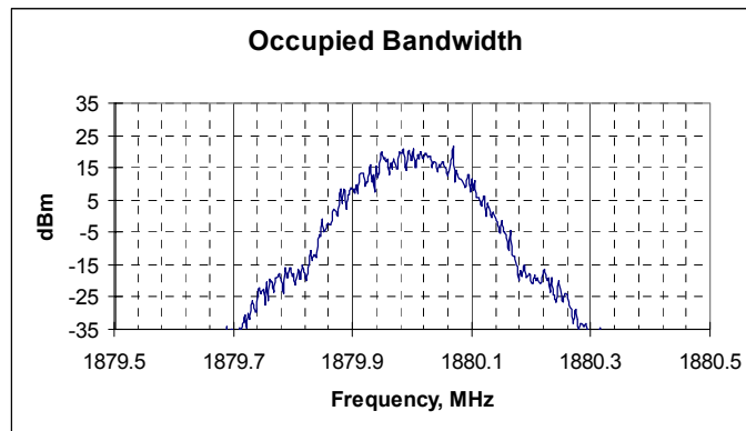
Picture 4. 99% occupied bandwidth, channel 661 GSM1900
