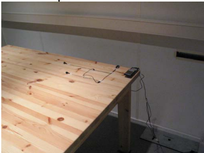
Picture 5 AC powerline conducted emission measurement, GSM
