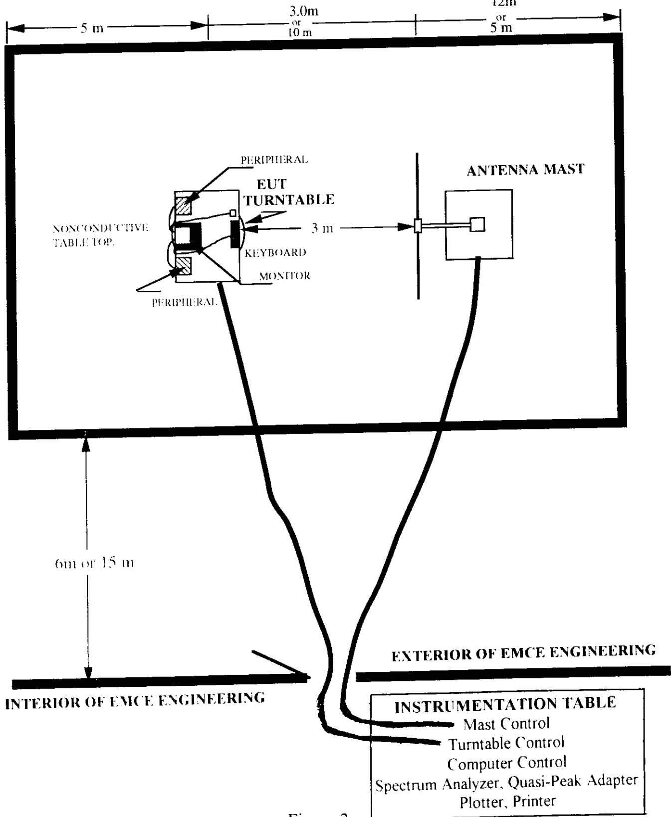
Figure 3 Radiated Emissions Test setup
