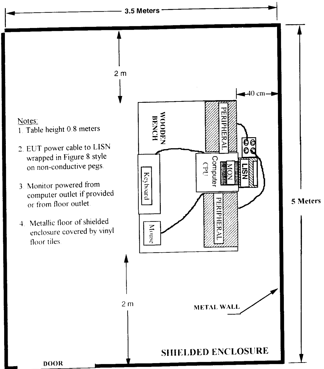
Figure 2 Conducted Emissions Test Setup
