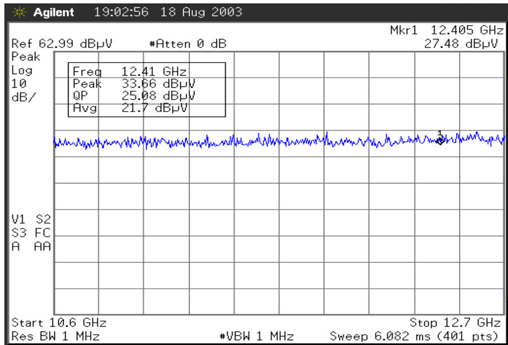
Plot #13 Antenna: UNI-28-5.8 P/N 872811
