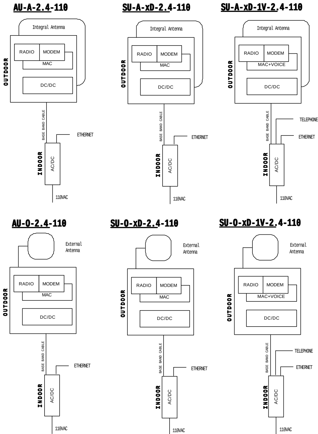
Fig. 1 BreezeAccess Products
