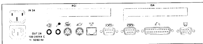
Figure 3 Rear Panel of the Thin Client with 16 Bit Stereo output
