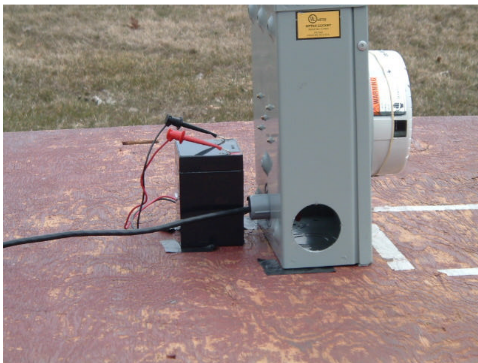
PICTORIAL 1 HEXAGRAM MODEL 10152 MTU OUTPUT POWER AND SPURIOUS EMISSIONS TYPICAL TEST SETUP
