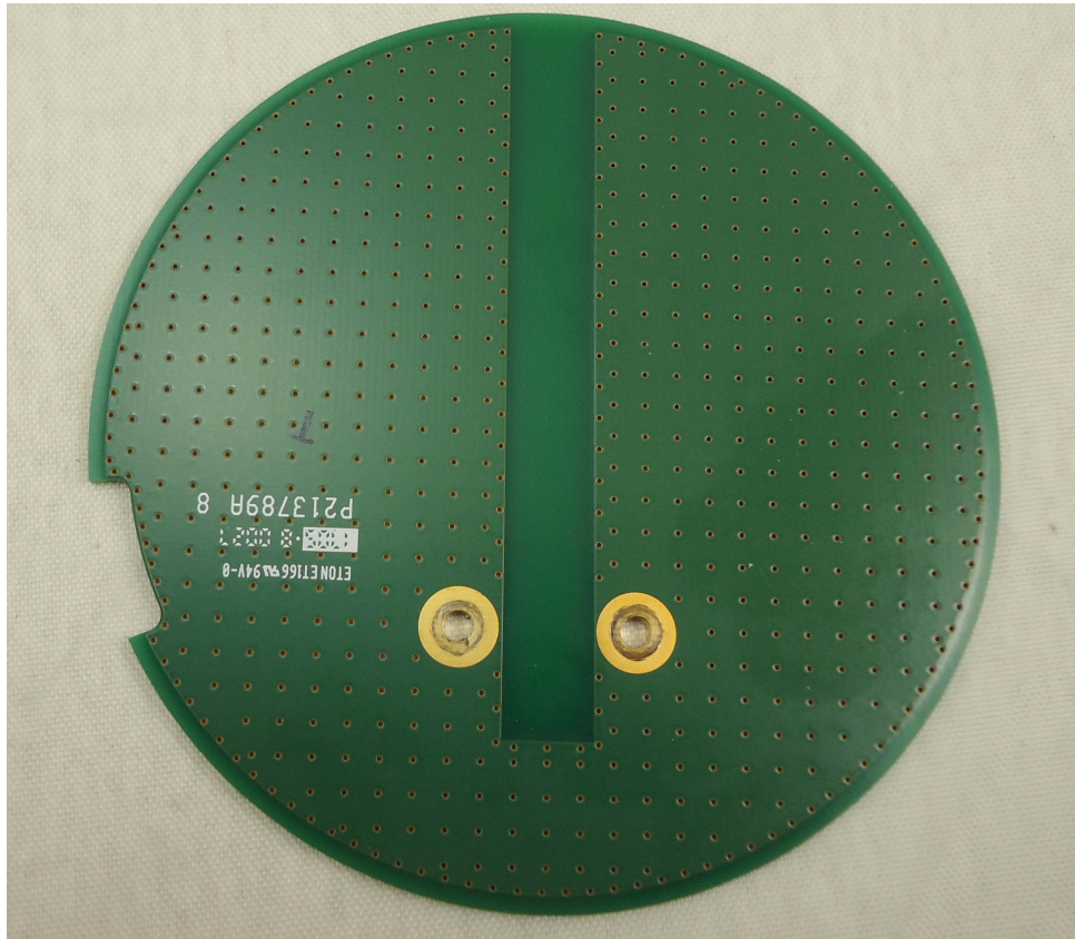
PCB Antenna
