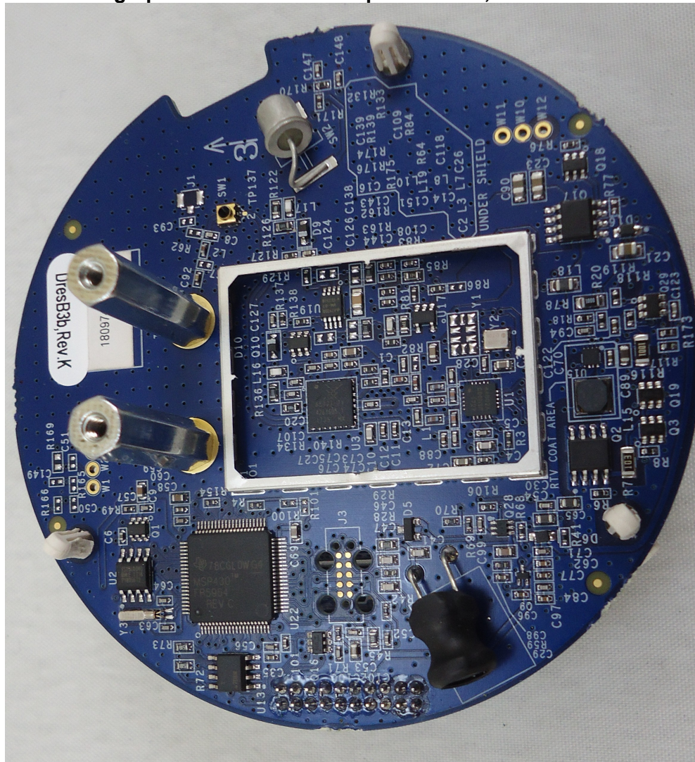
Photographs of PC Board: Component Side; Shield removed
