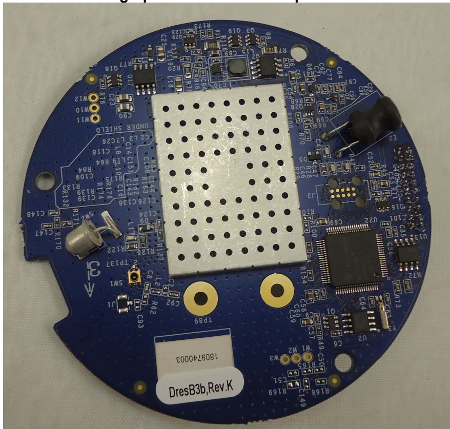
Photograph of PC Board: Component Side
