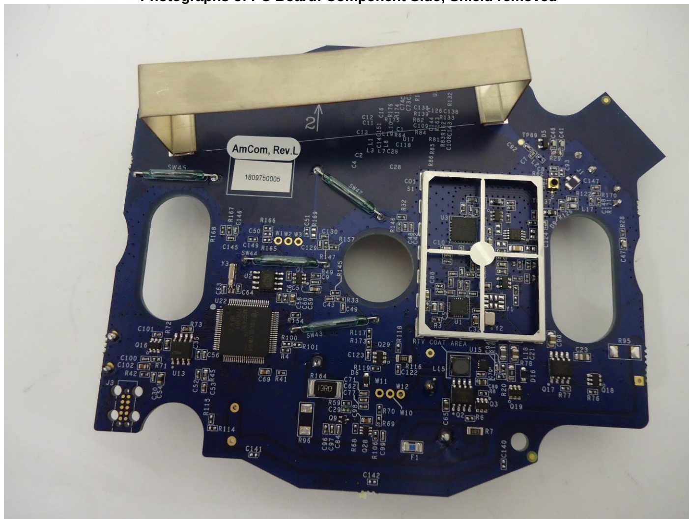
Photographs of PC Board: Component Side; Shield removed
