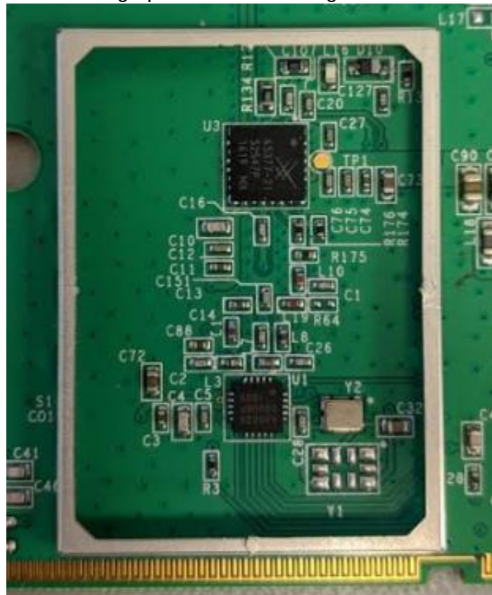
Photograph of PC Board: Cage Removed
