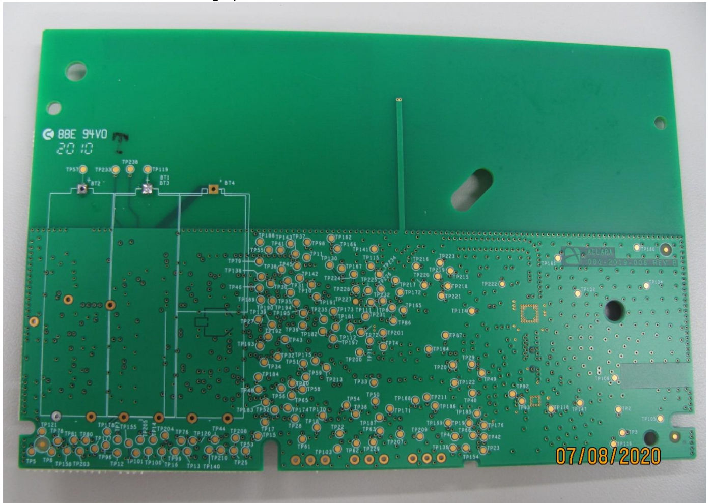
Photograph of PC Board: Foil Side, Batteries Removed
