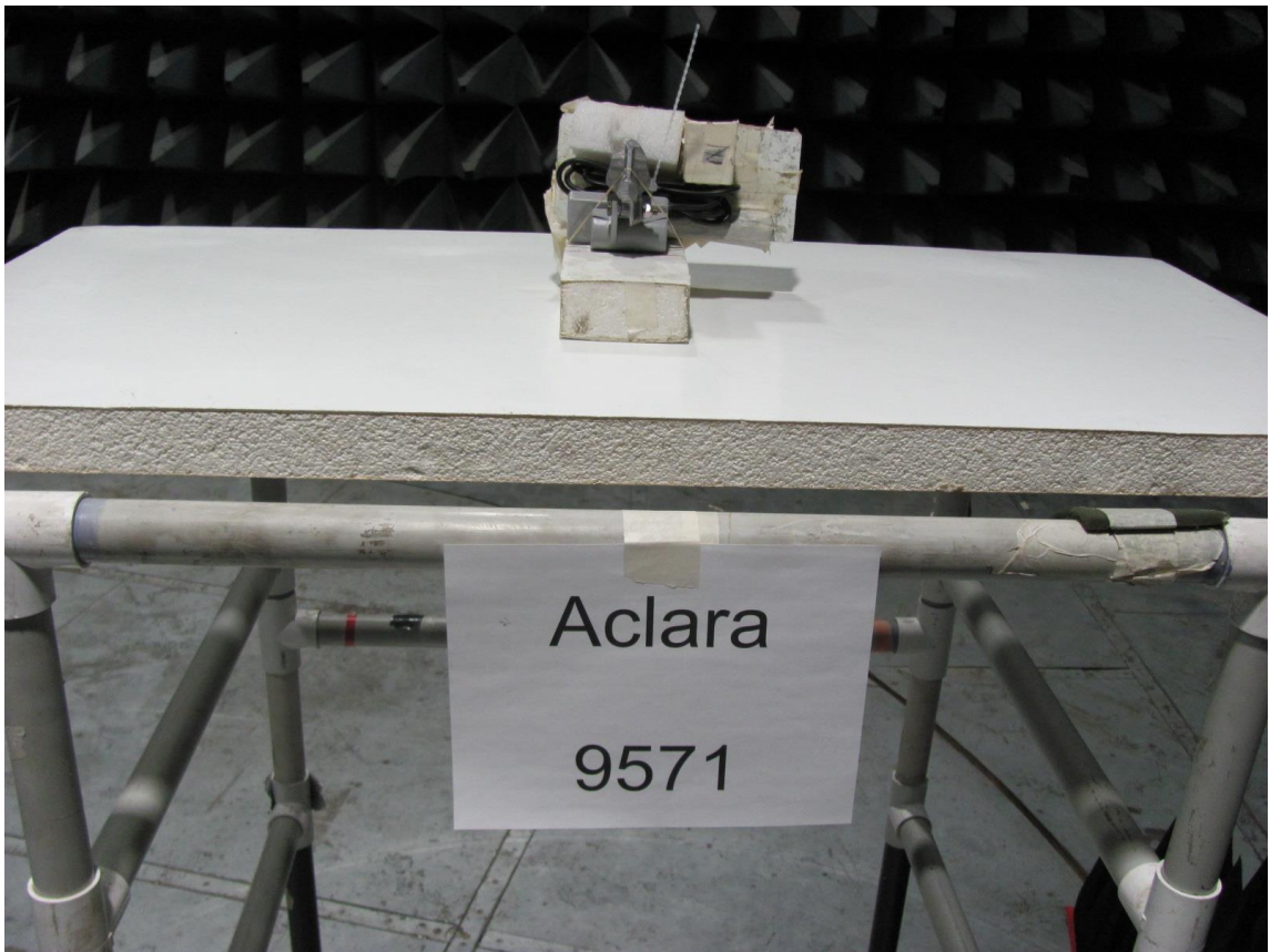
The EUT was taped to a foam stand in order to change its orientation
