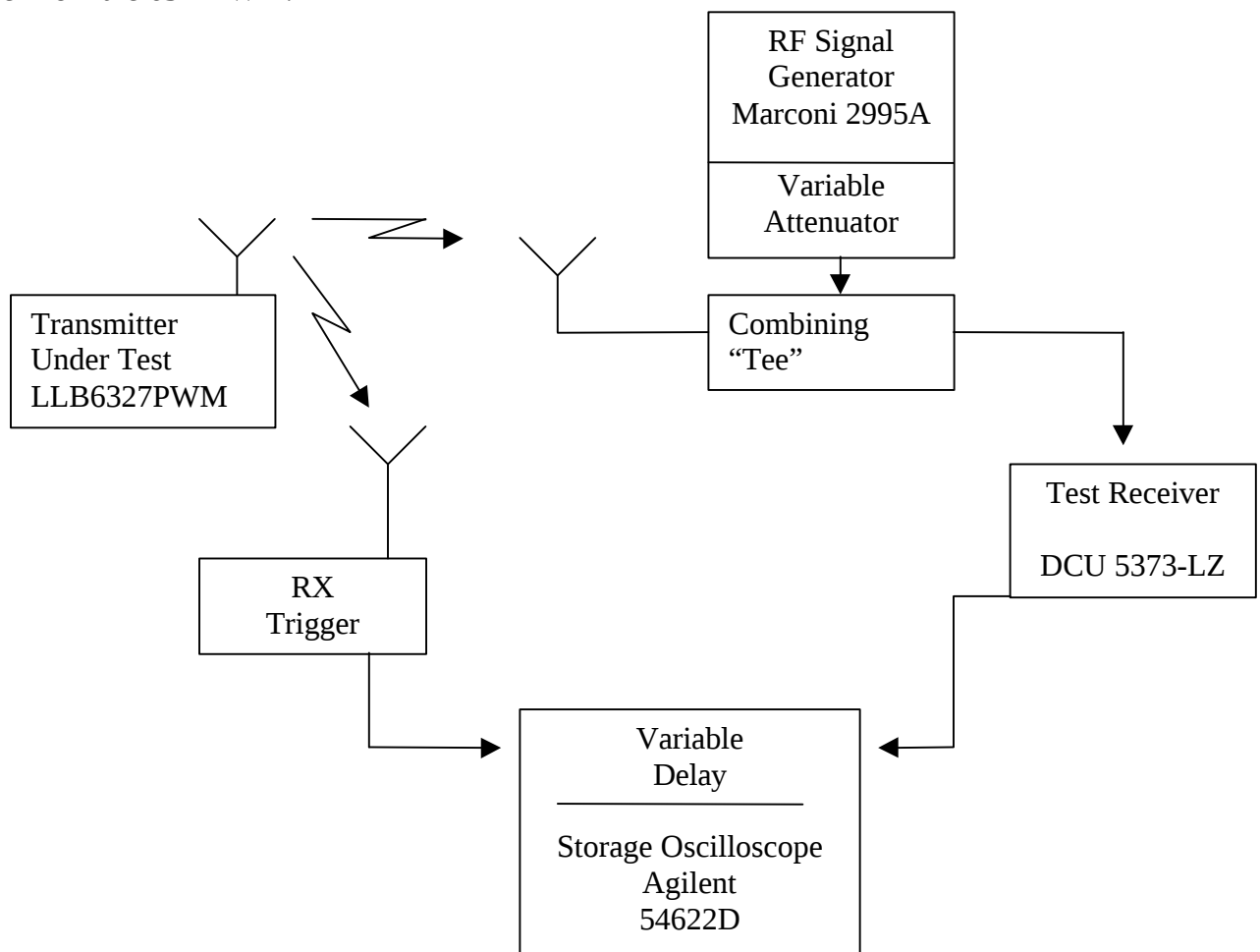
Fig. 2 Transient Frequency Behavior Test Setup
